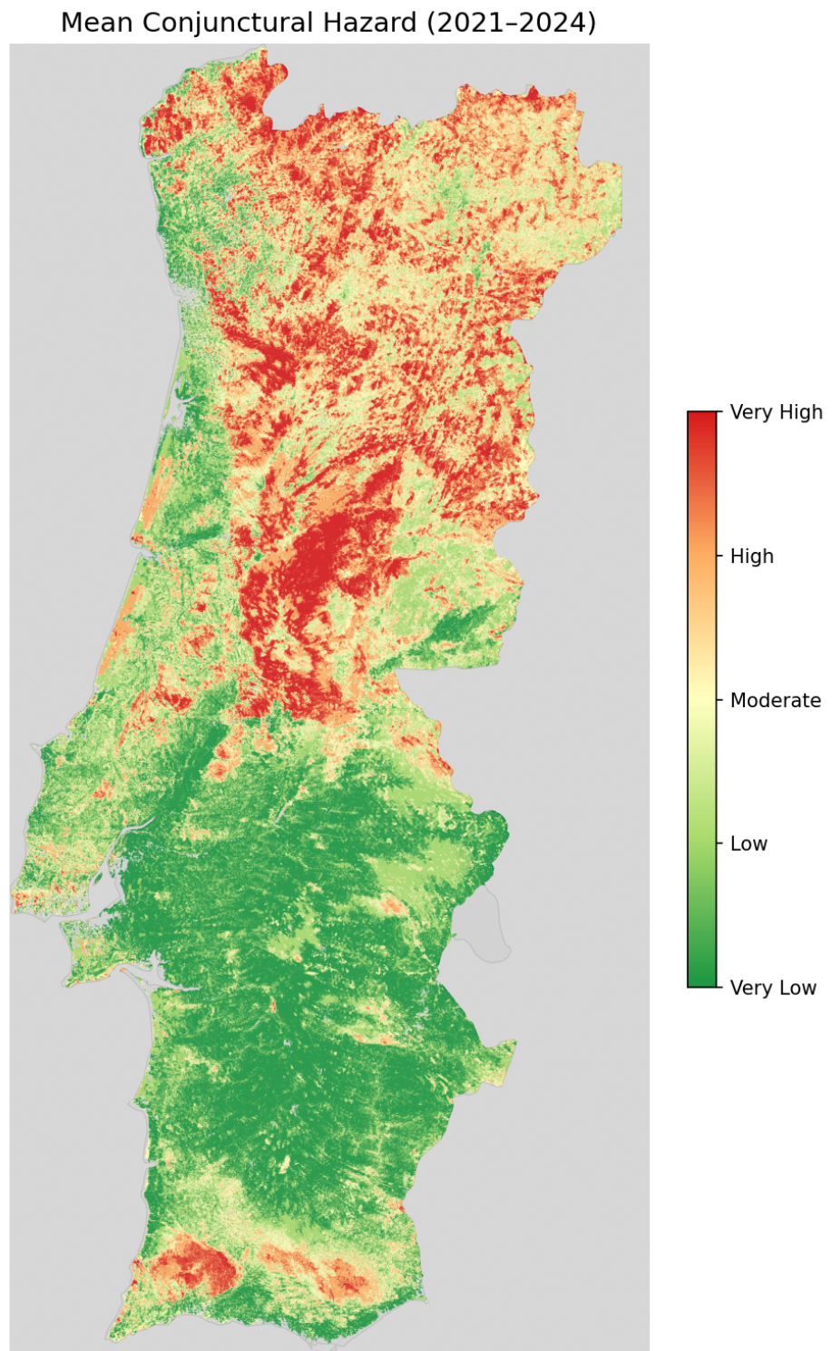
Figure 2: Mean conjunctural hazard index across mainland Portugal, 2021–2024.
