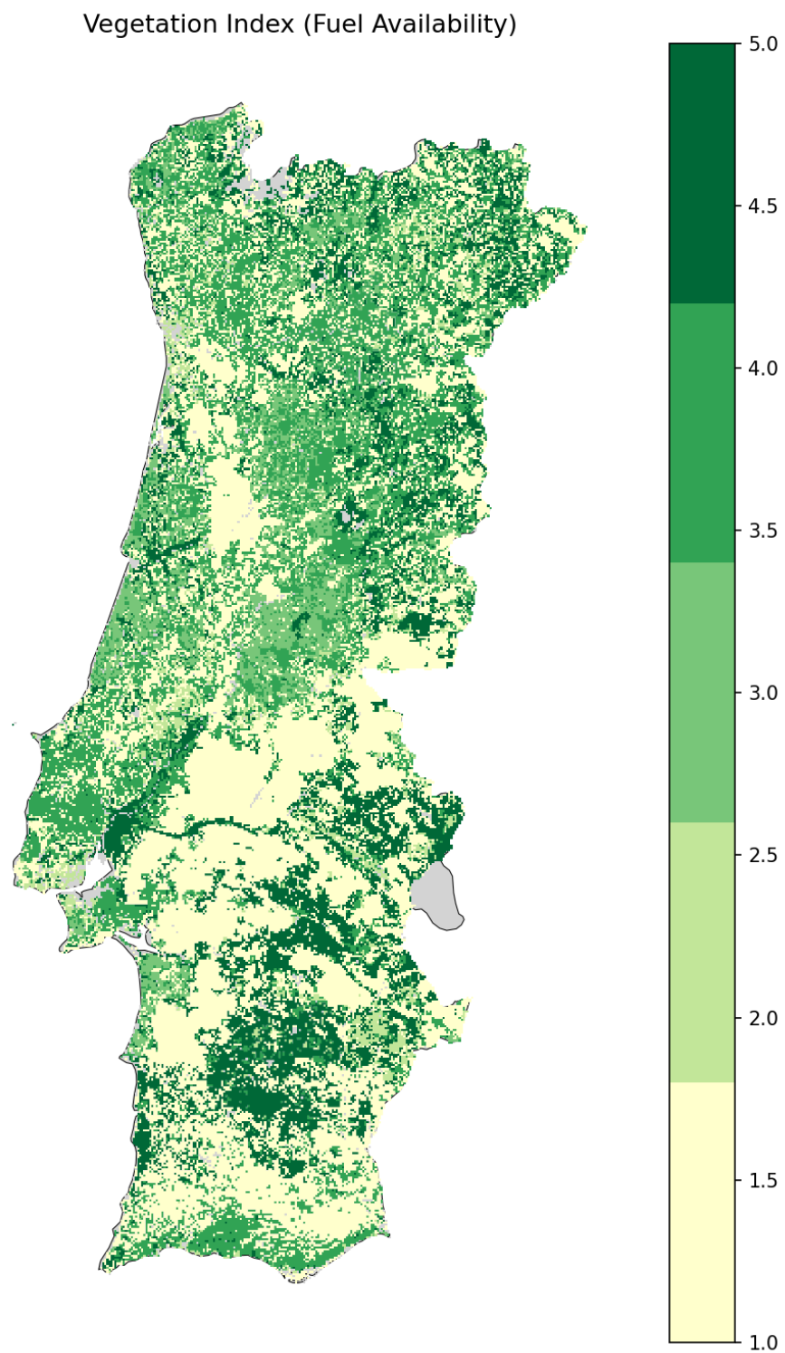
Figure 3: Vegetation index (IQV) across mainland Portugal.
