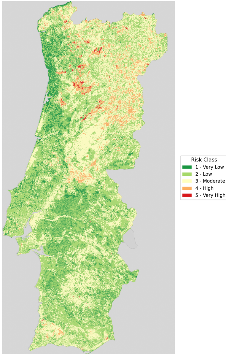
Integrated Wildfire Risk Model — Portugal (2021–2024)
