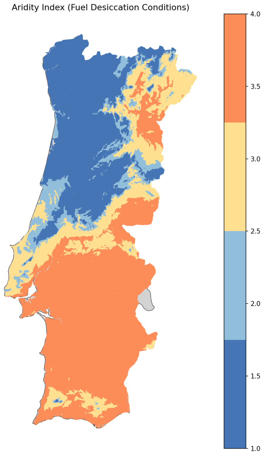
Figure 4: Aridity index across mainland Portugal.
