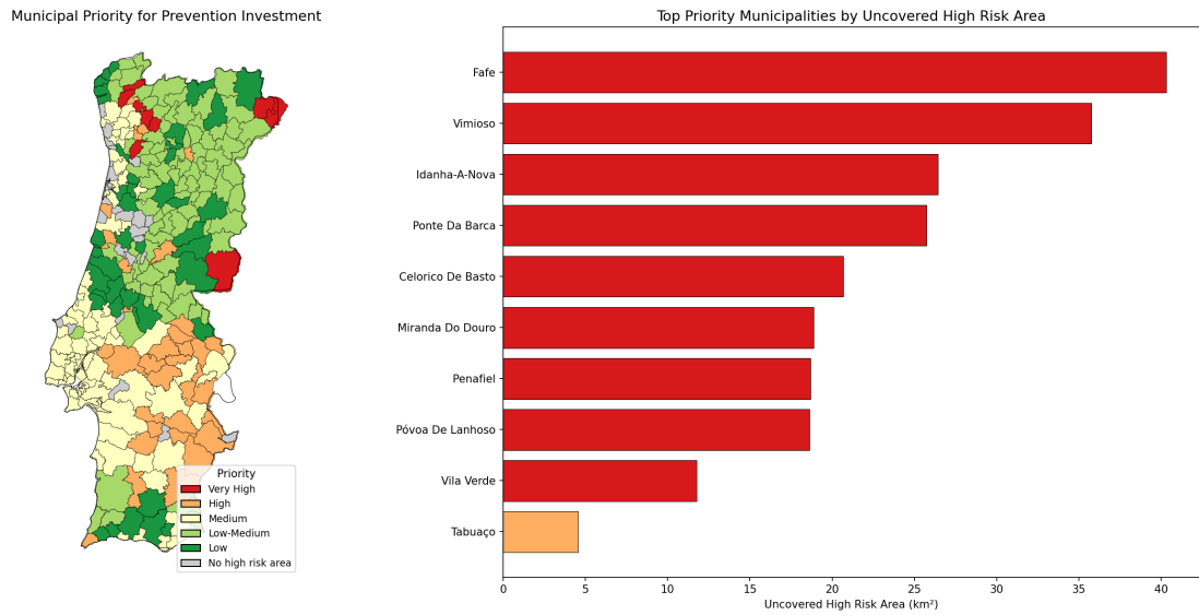
Figure 16: Left: Municipal priority classification for prevention investment. Right: Top priority municipalities by uncovered high-risk area (km 2 ).
