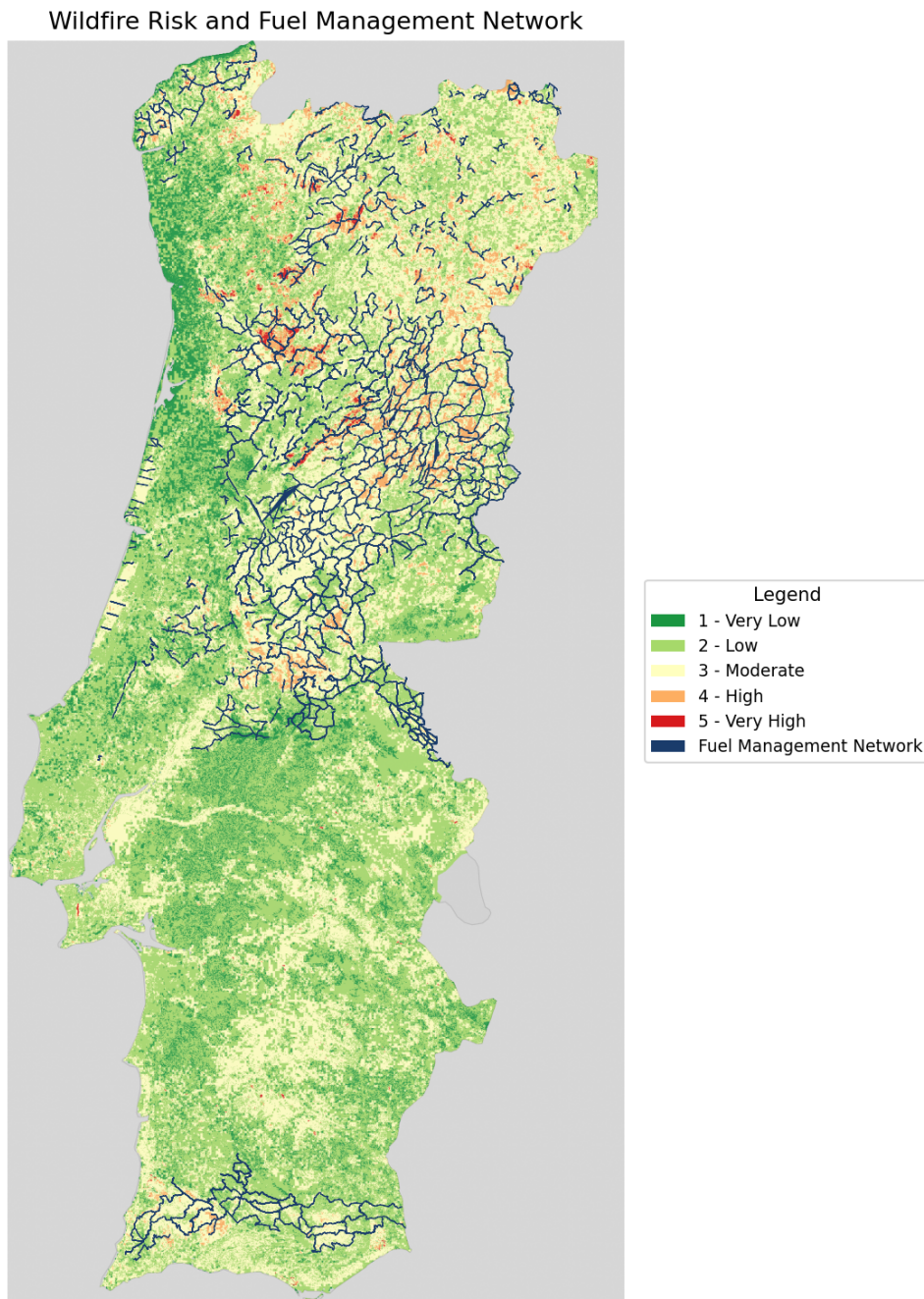
Figure 9: Spatial overlay of the integrated wildfire risk model and the Primary Fuel Management Network across mainland Portugal (2021–2024). Risk classes range from 1 (Very Low) to 5 (Very High). The network is shown in dark blue.
