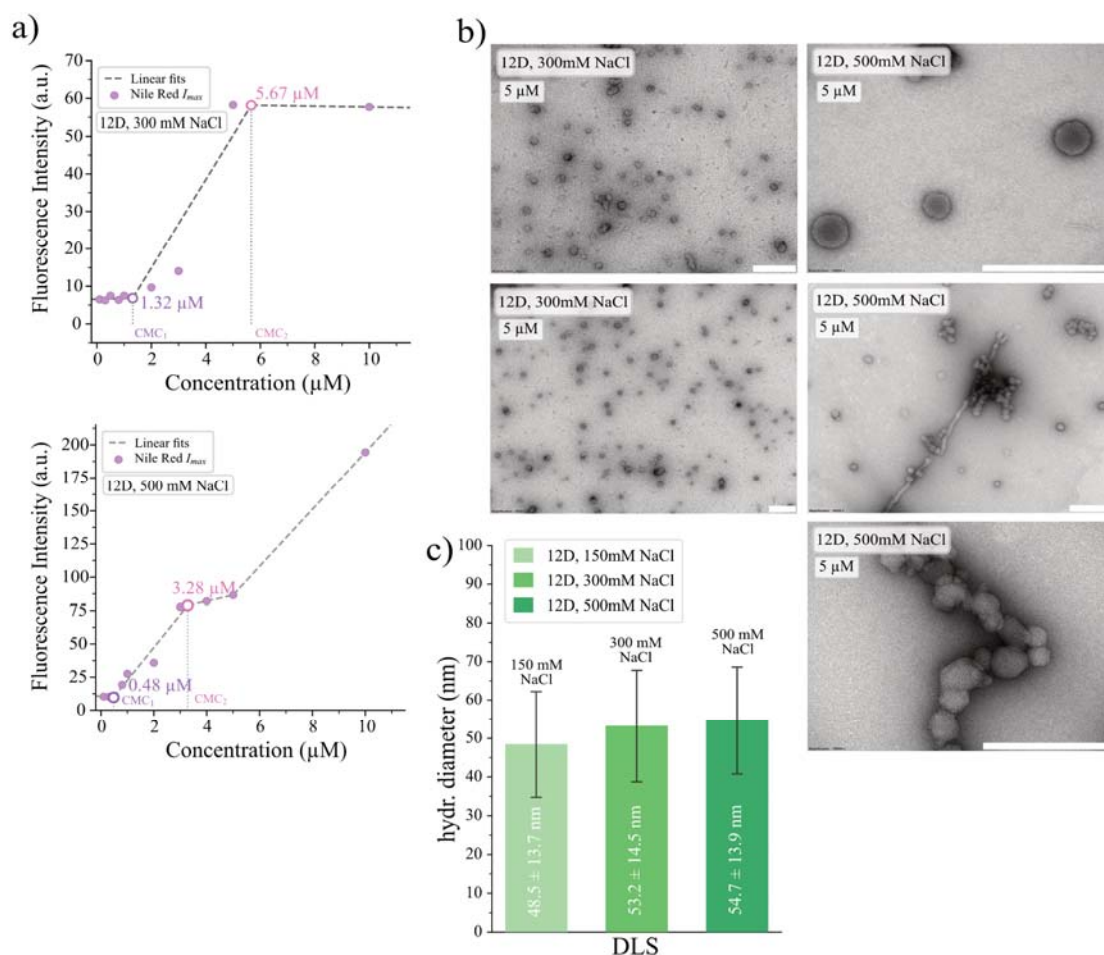
Figure 9. Salt-dependent self-assembly of phosphomimetic 12D TDP43-LCD. a) Nile Red fluorescence intensity versus protein concentration for 12D LCD at 300 mM NaCl (top) and 500 mM NaCl (bottom), showing two distinct CMC transitions at high salt b) Negative-stain TEM images of 5 \mu\text{M} 12D at 300 mM NaCl (spherical micelles) and 500 mM NaCl (spherical and worm-like structures). c) Mean hydrodynamic diameters of 5 \mu\text{M} 12D determined by DLS at 150, 300 and 500 mM NaCl (mean \pm s.d., n = 12 ).
