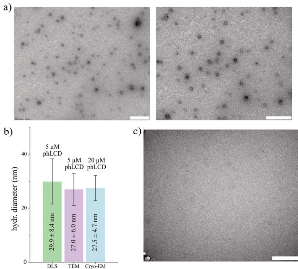
Figure 5. Direct visualization of phosphorylated TDP-43 LCD micelles by negative-stain TEM and cryo-EM confirms a uniform spherical architecture with native diameters of ~30 nm. a) Representative negative-stain TEM images of 5 \mu M phLCD in 150 mM NaCl conditions, showing spherical nanoparticles. Scale bar, 300 nm. b) Direct comparison of mean micelle diameters obtained by three orthogonal methods: DLS (peak maximum of the intensity-weighted hydrodynamic diameters distribution; 5 \mu M phLCD, n = 12 biological replicates), negative-stain TEM (5 \mu M phLCD, >200 particles analyzed), and cryo-EM in vitreous ice (20 \mu M phLCD, n > 100 particles). Bars indicate mean \pm s.d. c) Representative cryo-EM micrograph of phLCD at 20 \mu M in vitreous ice, showing well-dispersed spherical particles consistent with the negative-stain TEM and DLS measurements. Scale bar, 300 nm.
