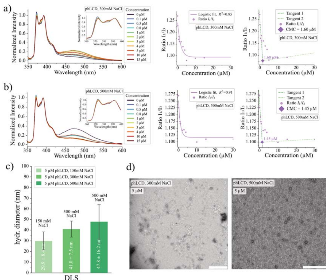
Figure 8. Salt-dependent self-assembly of phosphorylated TDP-43 LCD. a) Determination of critical micelle concentration using pyrene. Left: normalized fluorescence emission spectra at increasing phLCD concentrations at 300 mM NaCl buffer. Right: Ratio of pyrene vibronic bands ( I_1/I_3 ) plotted against phLCD concentration, fitted with a logistic function ( R^2 = 0.85 ) and tangent lines indicating CMC \approx 1.60 \mu\text{M} . b) Determination of critical micelle concentration using pyrene. Left: normalized fluorescence emission spectra at increasing phLCD concentrations at 500 mM NaCl buffer. Right: Ratio of pyrene vibronic bands ( I_1/I_3 ) plotted against phLCD concentration, fitted with a logistic function ( R^2 = 0.91 ) and tangent lines indicating CMC \approx 1.45 \mu\text{M} . c) Mean hydrodynamic diameters of 5 μM phLCD determined by DLS at 150, 300 and 500 mM NaCl (mean \pm s.d., n = 12 ). d) Representative negative-stain TEM micrographs of 5 μM phLCD at 300 mM and 500 mM NaCl. Scale bar, 300 nm.
