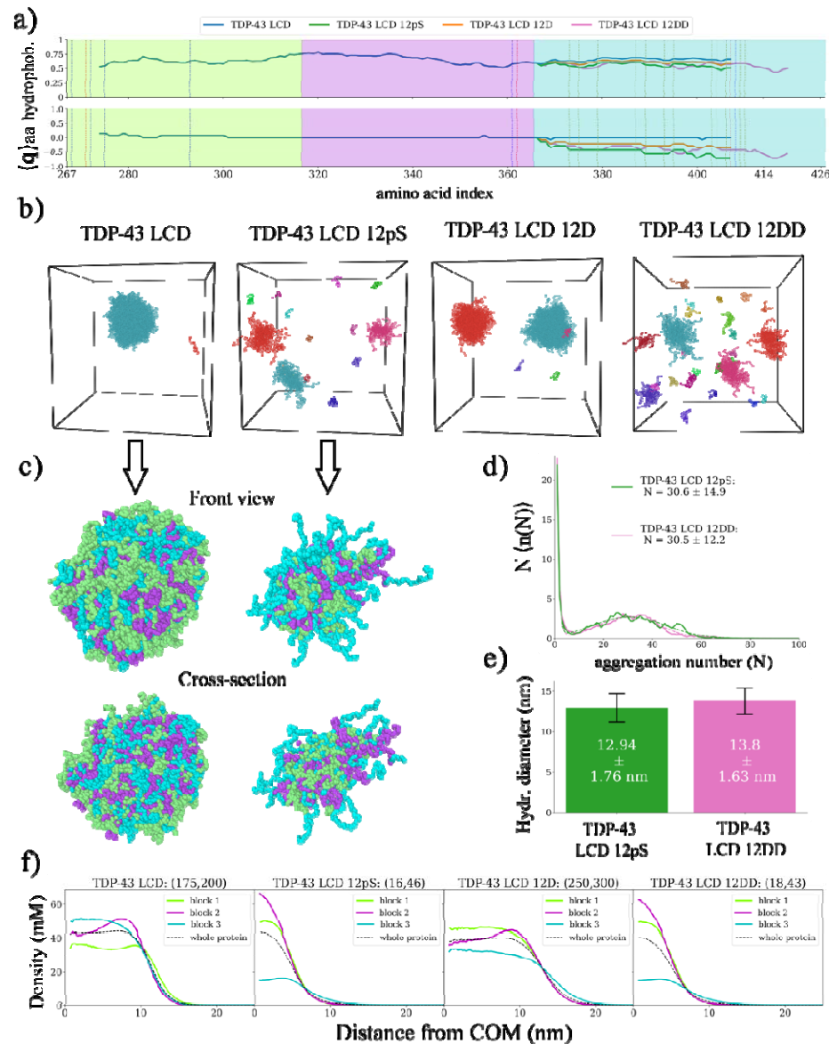
Figure 2. Coarse-grained simulations predict phosphorylation-induced micellization in TDP-43 LCD. a) Sliding average of mean hydrophobicity (top) and net charge per residue (bottom) along the sequence. The sequence is divided into 3 blocks of nearly identical length, shown in cyan, pink, and light green, representing the C-terminal, central, and N-terminal blocks. Dashed lines indicate sequence charges, blue and red represent positive and negative charges, respectively, and olive lines represent phosphorylation sites. b) Snapshots of simulation trajectories. Different colours represent different clusters. A zoomed-in snapshot of a TDP-43 LCD 12pS micelle is shown next to them. A front view and a cross-sectioned (sliced in half) view are provided. Amino acids are coloured according to the colour-coding in a and f. They provide a visualisation of the segregated internal architecture of the micelles. c) Zoomed-in snapshots of TDP-43 LCD and TDP-43 LCD 12pS assemblies. A frontal view and a cross-sectioned (sliced in half) view are provided. Amino acids in different sequence blocks are coloured according to the colour-coding in a and f. d) Size distribution (full lines) and corresponding fitting curves (dashed lines) for the 2 sequences (TDP-43 LCD 12pS and 12DD) forming finite-sized structures. Mean aggregation number and standard deviation are shown in the legend. e) Mean hydrodynamic diameter for both micellizing sequences. Results were obtained as a weighted average of the hydrodynamic radii of clusters of sizes within one standard deviation of the mean aggregation number of the micelles, as determined from the fit to the size distributions. Error bars represent the standard deviation of the distribution of hydrodynamic
