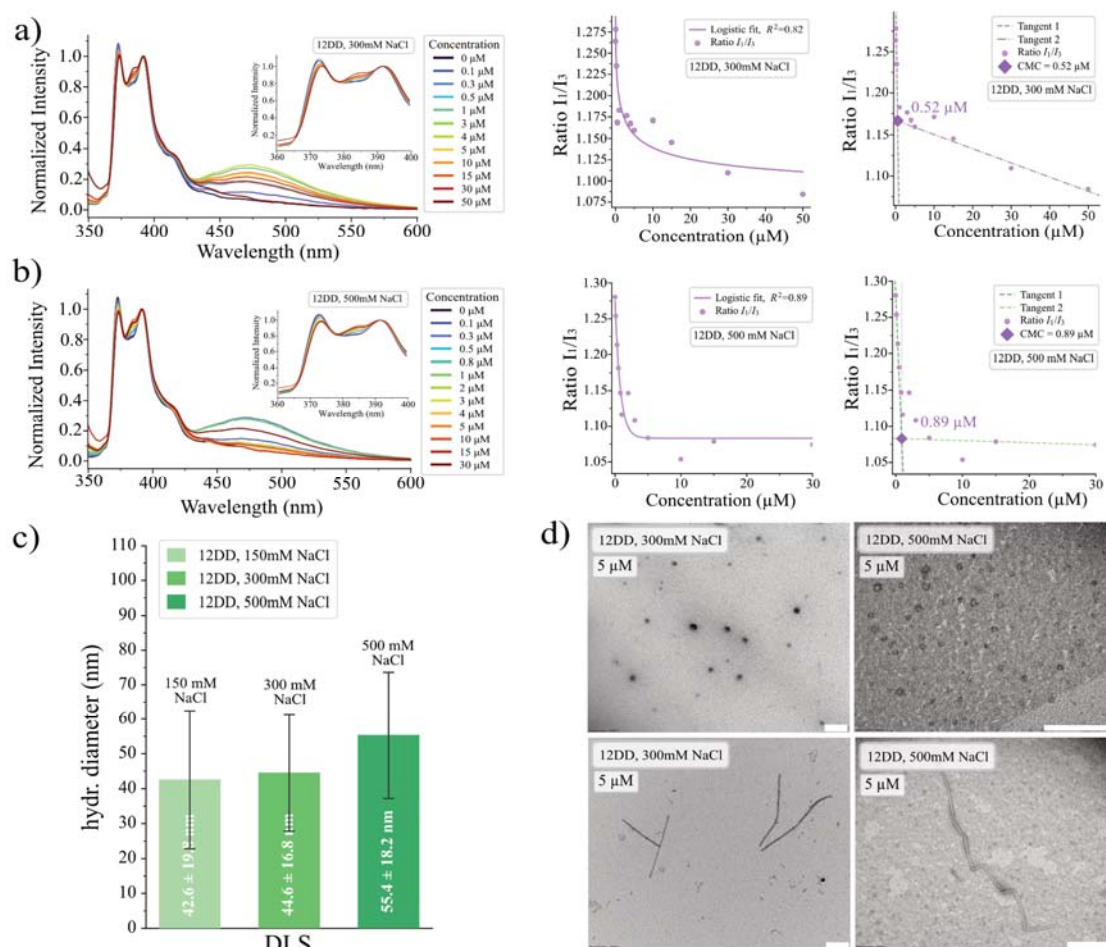
Figure 10. Salt-dependent self-assembly of phosphomimetic 12DD LCD. a) Determination of critical micelle concentration using pyrene. Left: normalised fluorescence emission spectra at increasing 12DD LCD concentrations at 300 mM NaCl buffer. Right: Ratio of pyrene vibronic bands ( I_1/I_3 ) plotted against 12DD LCD concentration, fitted with a logistic function ( R^2 = 0.82 ) and tangent lines indicating CMC \approx 0.52 \mu\text{M} . b) Determination of critical micelle concentration using pyrene. Left: normalised fluorescence emission spectra at increasing 12DD LCD concentrations at 500 mM NaCl buffer. Right: Ratio of pyrene vibronic bands ( I_1/I_3 ) plotted against 12DD LCD concentration, fitted with a logistic function ( R^2 = 0.89 ) and tangent lines indicating CMC \approx 0.89 \mu\text{M} . c) Mean hydrodynamic diameters of 5 \mu\text{M} 12DD LCD determined by DLS at 150, 300 and 500 mM NaCl (mean \pm s.d., n = 12 ). d) Negative-stain TEM images of 5 \mu\text{M} 12DD at 300 mM NaCl and 500 mM NaCl. Scale bar, 300 nm.
