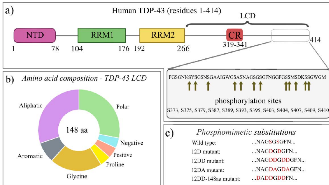
Figure 1. Full-length TDP-43 sequence. a) Representation of TDP-43 domains. The last 48 residues of the low complexity domain (LCD) are shown. The location of the phosphorylation sites relevant to this work are indicated by arrows. b) Amino acid composition of TDP-43 LCD. c) Schematic representation of the phosphomimetic substitution patterns used in this study, illustrated for a representative C-terminal sequence segment. In the wild-type sequence, the serine residues targeted for phosphorylation are highlighted in red. In the 12D mutant, each of the 12 target serines is replaced by a single aspartate (S→D), preserving the wild-type LCD length of 148 residues and introducing a C-terminal block charge of -12e. In the 12DD mutant, each serine is replaced by two aspartates (S→DD), increasing the C-terminal block charge to -24e but extending the chain by 12 residues (160 residues total). Two additional control constructs were designed to disentangle charge from chain-length effects: the 12DA mutant, a length-matched analogue of 12DD (160 residues) in which one aspartate of each pair is replaced by alanine to restore the -12e charge of 12D while retaining the longer backbone; and the 12DD-148aa mutant, a length-matched analogue of 12D in which native residues adjacent to the substitution sites are removed to restore the wild-type LCD length of 148 residues while preserving the -24e charge. Substituted residues are shown in red.
