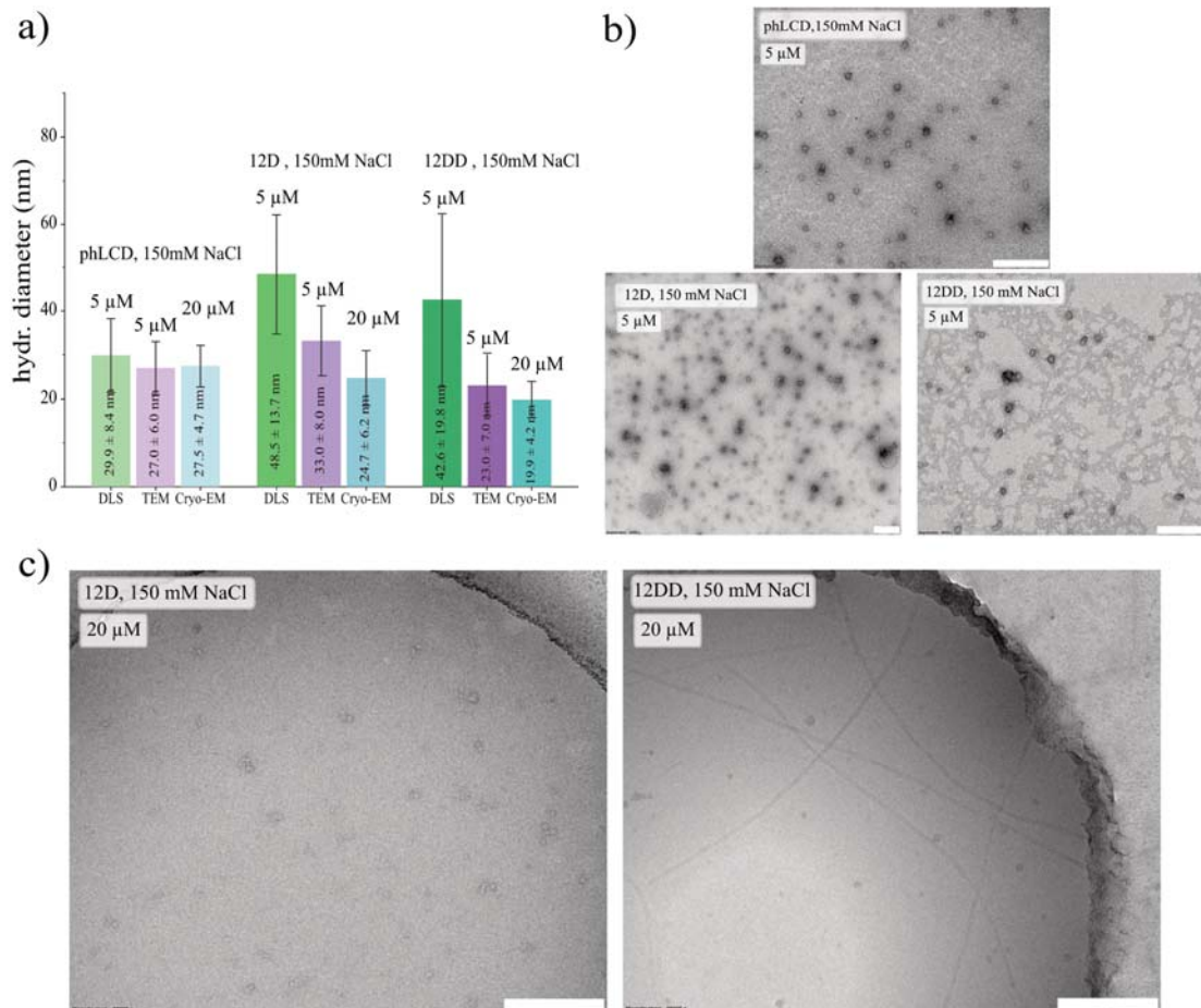
Figure 6. Phosphomimetic substitutions 12D and 12DD fully recapitulate the phenotype of phosphorylated TDP-43 LCD, forming stable spherical micelles of defined size above a low-micromolar critical micelle concentration. a) Direct comparison of mean diameters obtained by dynamic light scattering (DLS, 173° backscattering geometry, peak maximum of the intensity-weighted size distribution, n = 12 biological replicates), negative-stain TEM ( >200 particles per construct) and cryo-EM in vitreous ice ( >100 particles per construct) for phLCD, 12D and 12DD in physiological buffer (150 mM NaCl, pH 7.5, 25 °C). DLS and TEM measurements were performed at 5 μM; cryo-EM at 20 μM. Data are mean ± s.d. b) Representative negative-stain TEM images at 5 μM for phLCD (upper), 12D (lower left), and 12DD (lower right). Scale bars, 300 nm. c) Representative cryo-EM micrographs at 20 μM for 12D (left) and 12DD (right). The 12DD sample additionally shows occasional thin fibrillar structures coexisting with the dominant spherical micellar population - a minor subpopulation not detected by negative-stain TEM at 5 μM, indicating that, unlike phLCD, the doubly-charged 12DD phosphomimetic does not fully abolish access to fibrillar morphologies. Scale bars, 300 nm.
