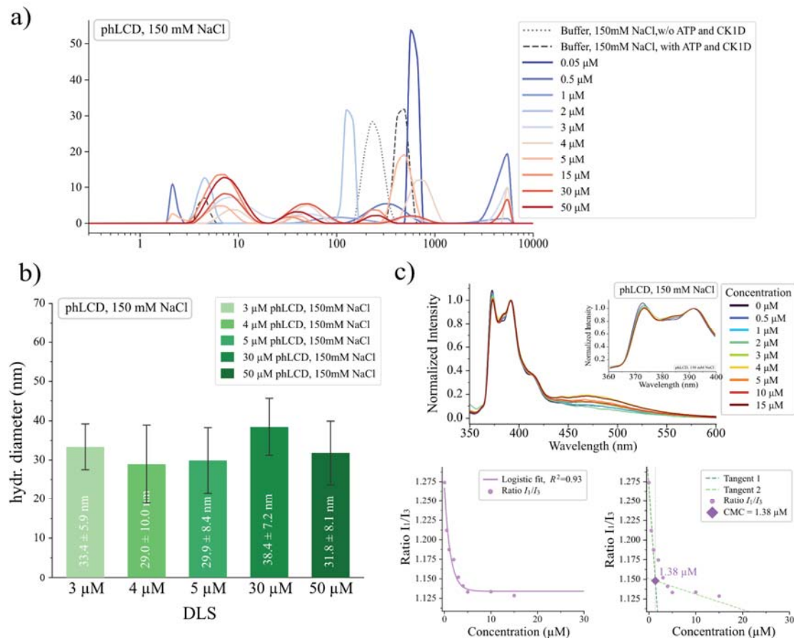
Figure 4. Phosphorylated TDP-43 LCD forms discrete, concentration-independent spherical assemblies with a low-micromolar critical micelle concentration. a) Intensity-weighted hydrodynamic diameter distributions of phLCD at concentrations ranging from 0.05 to 50 \mu\text{M} , together with two buffer controls: buffer alone (no protein, no kinase, no ATP) and buffer supplemented with CK1 \delta and ATP but lacking protein. A stable population centred around 30 nm is observed across the entire concentration range and is absent from both controls. b) Mean hydrodynamic diameters extracted from the protein-assembly peak of the DLS distributions in panel a for selected concentrations (3, 4, 5, 30 and 50 \mu\text{M} phLCD; mean \pm s.d., n = 12 ). c) Determination of critical micelle concentration using pyrene. Upper panel: normalized fluorescence emission spectra at increasing phLCD concentrations. Lower panel: Ratio of pyrene vibronic bands ( I_1/I_3 ) plotted against phLCD concentration, fitted with a logistic function ( R^2 = 0.93 ) and tangent lines indicating CMC \approx 1.38 \mu\text{M} .
