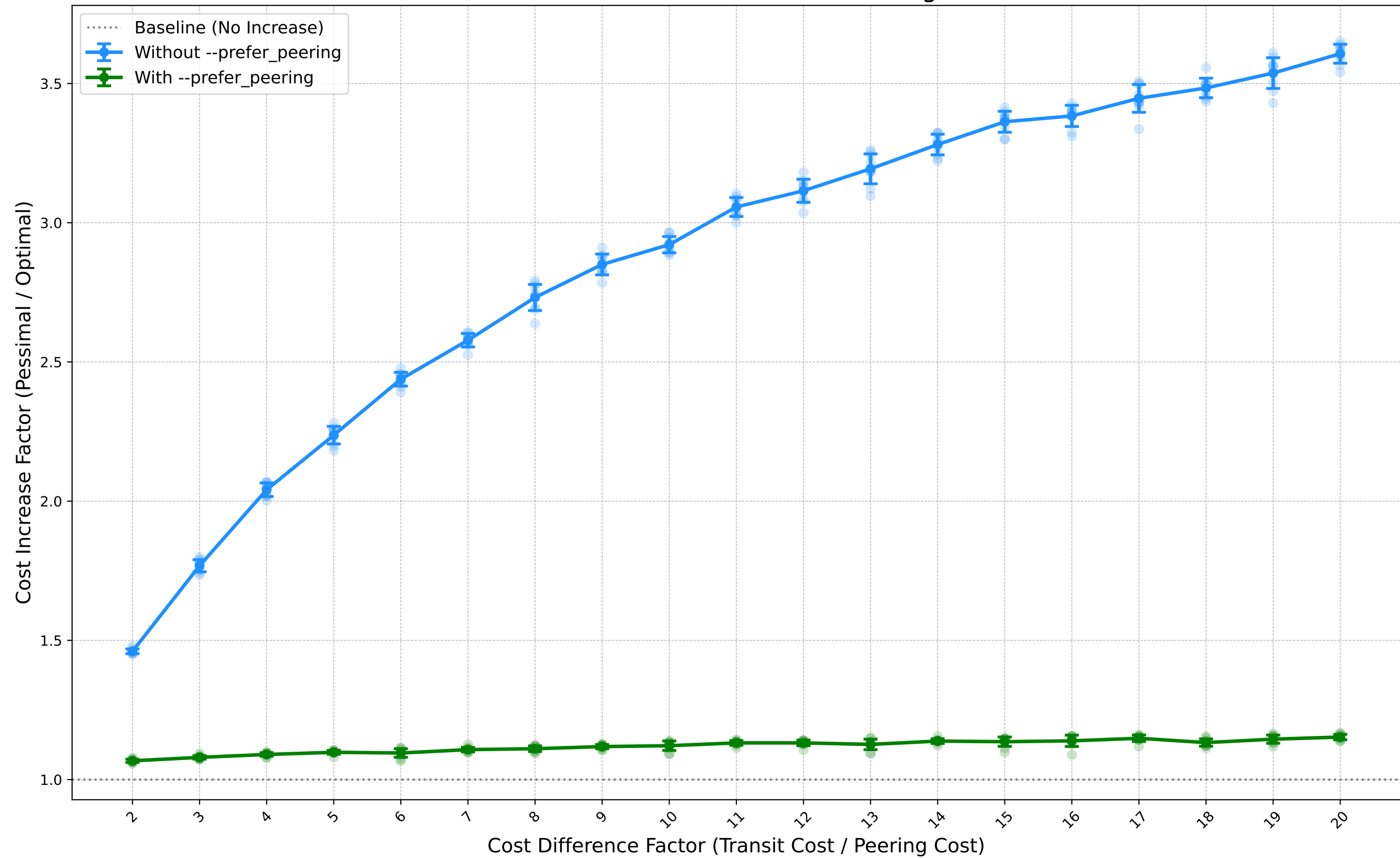
ISP Cost Increase: With vs. Without Peering Preference
