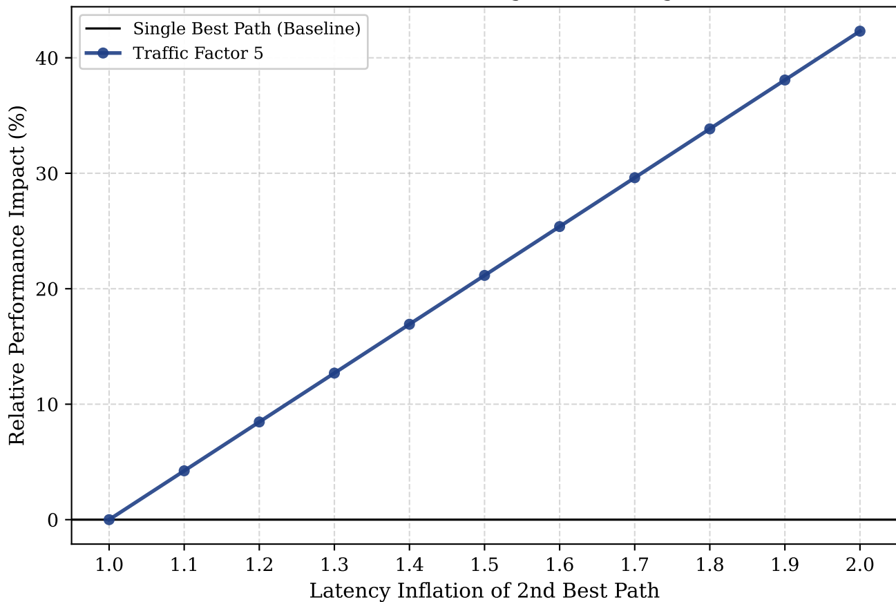
ECMP-2 Performance vs. Single Path (Range 1.0-2.0)
