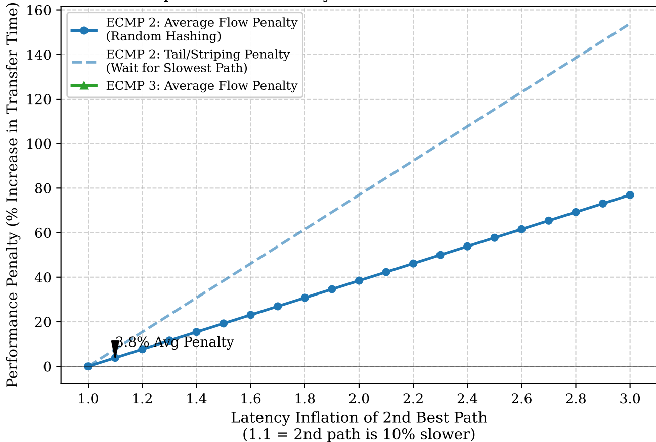
Impact of Path Latency Differences on Data Transfer
