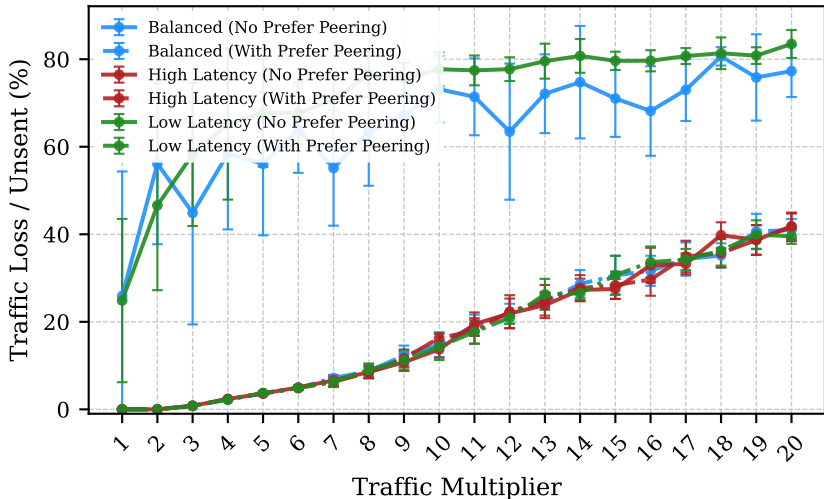
Packet Loss: waterfilling_optimal_1
