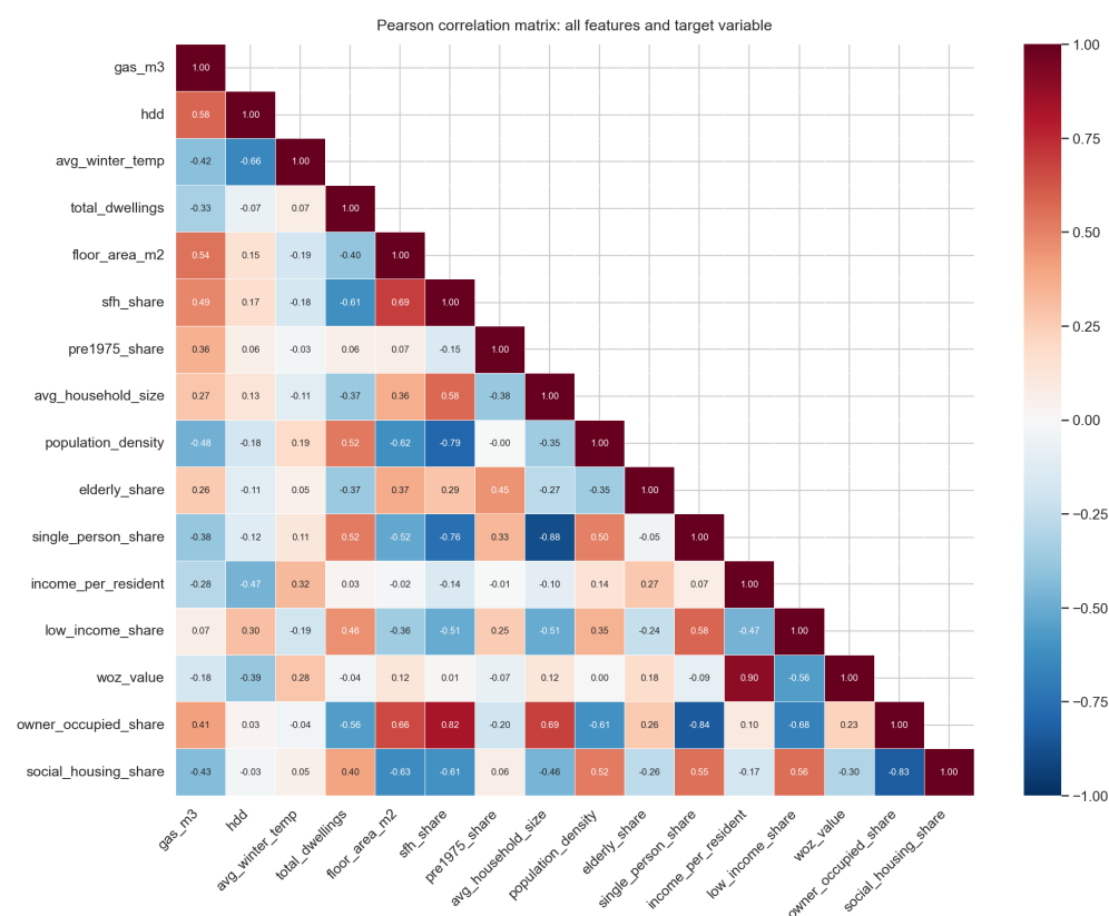
Figure 4. Pearson correlation matrix over the full 2016–2023 panel, covering the target ( gas_m3 ), the 14 model predictors, and total dwellings. Color and value give the correlation coefficient.
