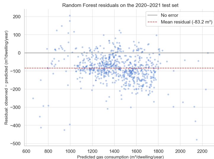
Figure 6. Random Forest residuals (observed minus predicted) on the 2020–2021 test set, plotted against predicted consumption. The solid line marks zero error and the dashed line the mean residual of -83.2 \text{ m}^3 . Most points lie below zero, showing a small and fairly even overprediction.
