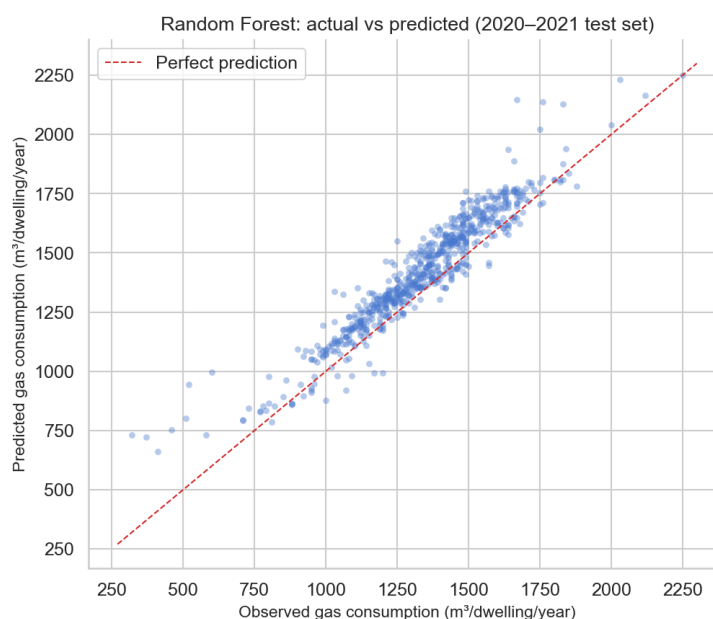
Figure 5. Random Forest predicted versus observed municipal gas consumption on the 2020–2021 test set. The dashed line marks perfect prediction.
