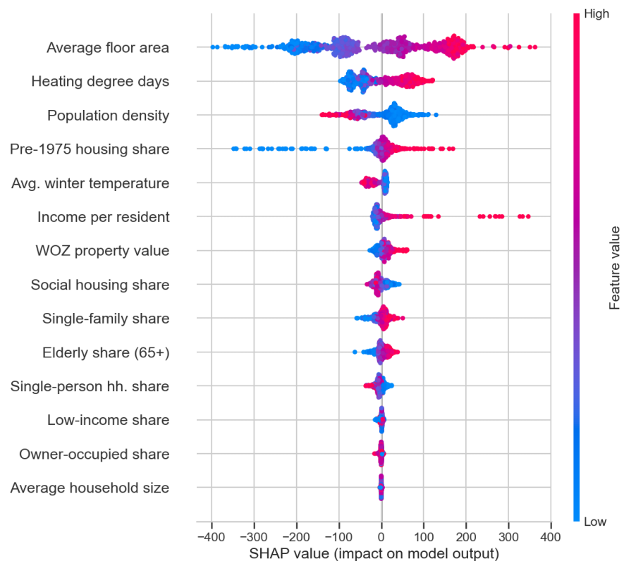
Figure 7. SHAP beeswarm plot for the Random Forest model on the 2020–2021 test set. Features are ordered top to bottom by mean absolute SHAP value. Each point is one municipality-year observation; horizontal position is the SHAP value in \text{m}^3 per dwelling per year, and color encodes the feature value from low (blue) to high (red).
