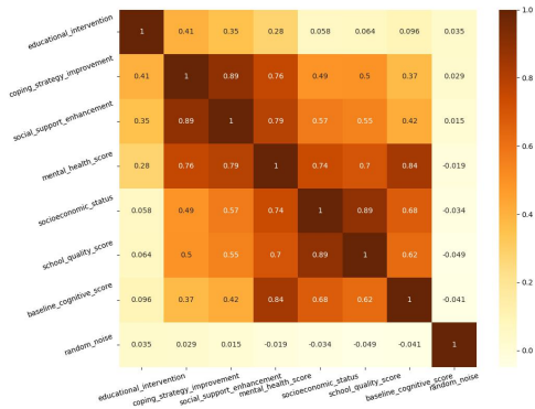
Correlation Matrix
