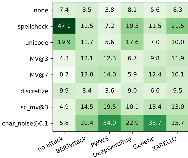
action × attacker
