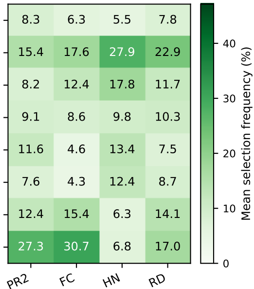
action × task
