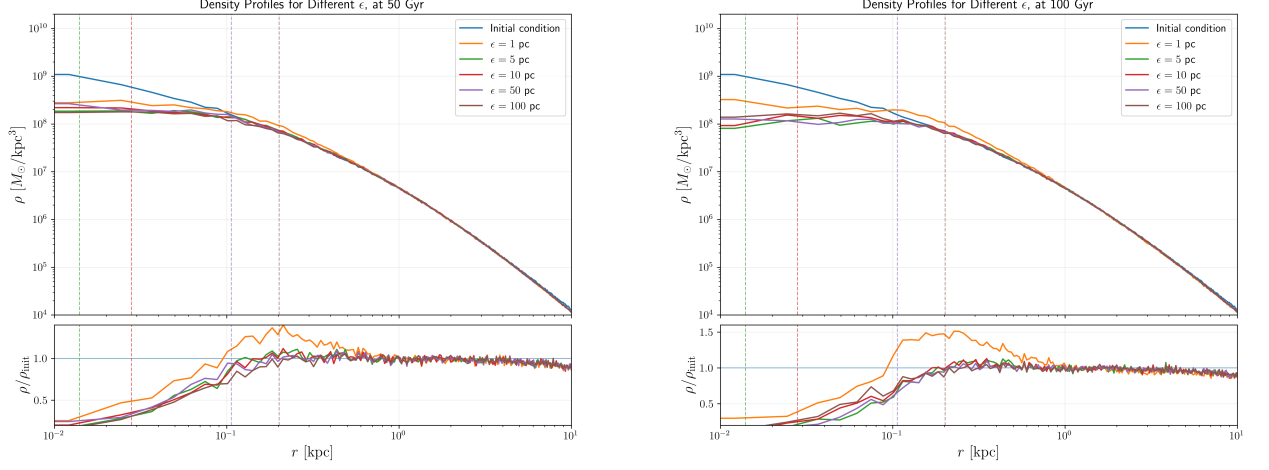
Figure 4.5: Softening study. Comparison of the same set of tested softening lengths at 50 Gyr (left) and 100 Gyr (right). The shorter-time view highlights the earlier evolution, while the longer-time view shows that the same hierarchy of softening runs follows the same qualitative trend. The smallest softening still shows a slight central-density increase close to the center, which is better interpreted as numerical heating than as a real improvement of the physical problem.
