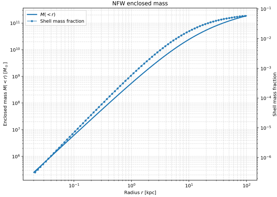
Figure 4.7: NFW enclosed mass and shell mass fraction. Left axis: monotonically increasing enclosed mass M(<r) with radius. Right axis: shell mass fraction per logarithmic shell. The outer halo contains a substantial fraction of the total mass budget, indicating that it cannot be ignored when computing potential depths.
