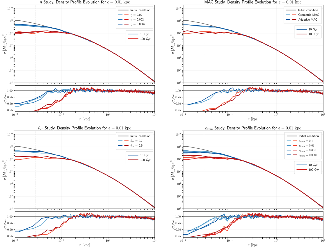
Figure 4.6: Self-gravity parameter study. Panels show the central-density evolution for the tested solver settings: top-left – timestep factor \eta (labelled ‘eta’); top-right – MAC choice; bottom-left – geometric opening angle \theta_{\text{cr}} ; bottom-right – FMM tolerance \epsilon_{\text{fmm}} . In each panel blue curves correspond to 10 Gyr and red curves to 100 Gyr.
