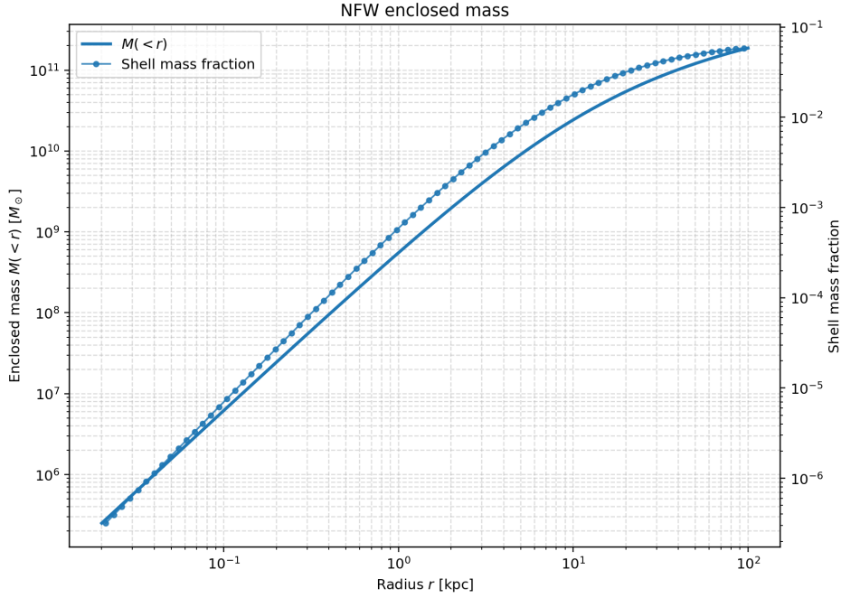
Figure 4.9: NFW enclosed mass and shell mass fraction. Left axis: monotonically increasing enclosed mass M(<r) with radius. Right axis: shell mass fraction per logarithmic shell. The outer halo contains a substantial fraction of the total mass budget, indicating that it cannot be ignored when computing potential depths.
