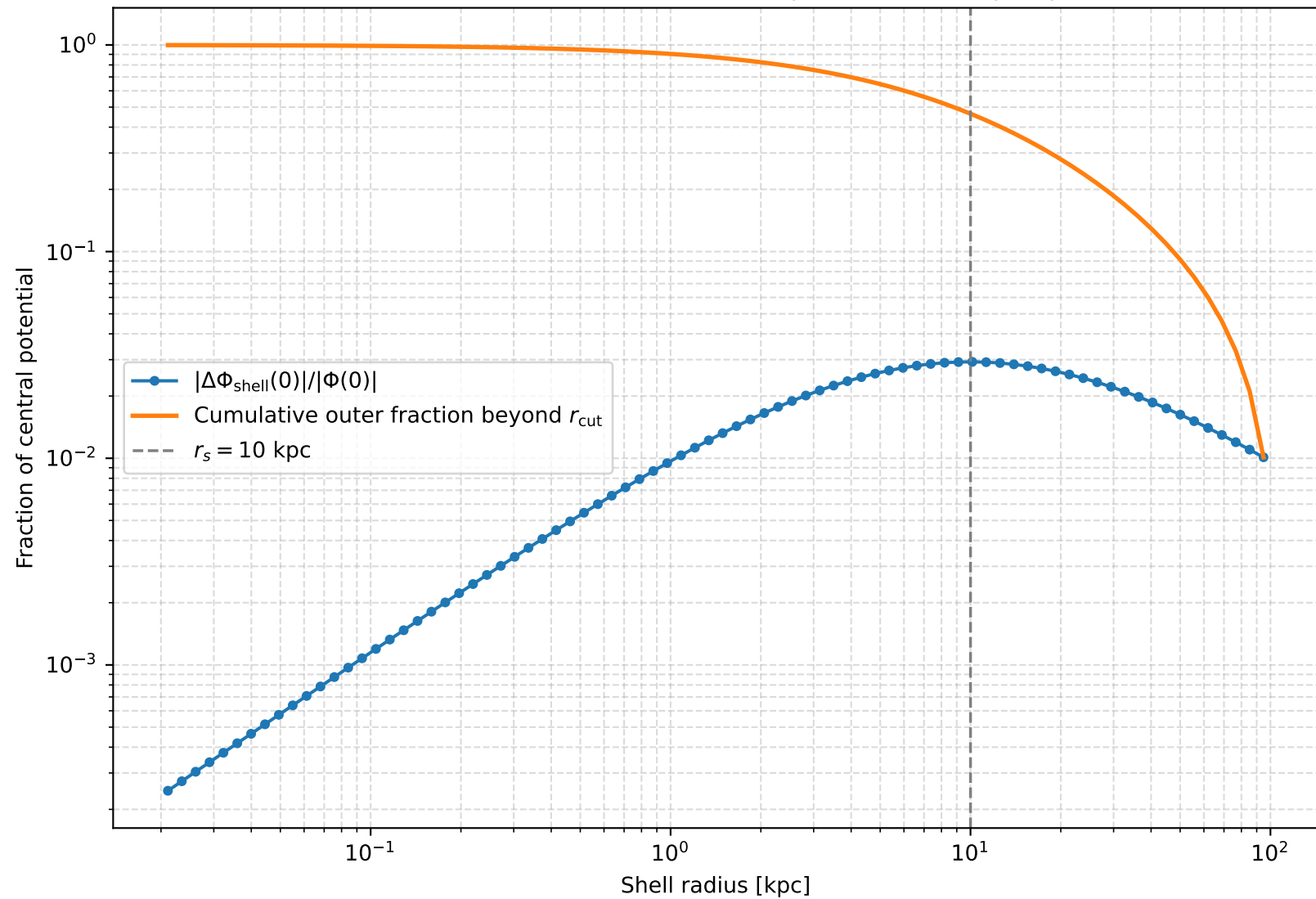
How each shell contributes to the central potential / escape-speed scale
