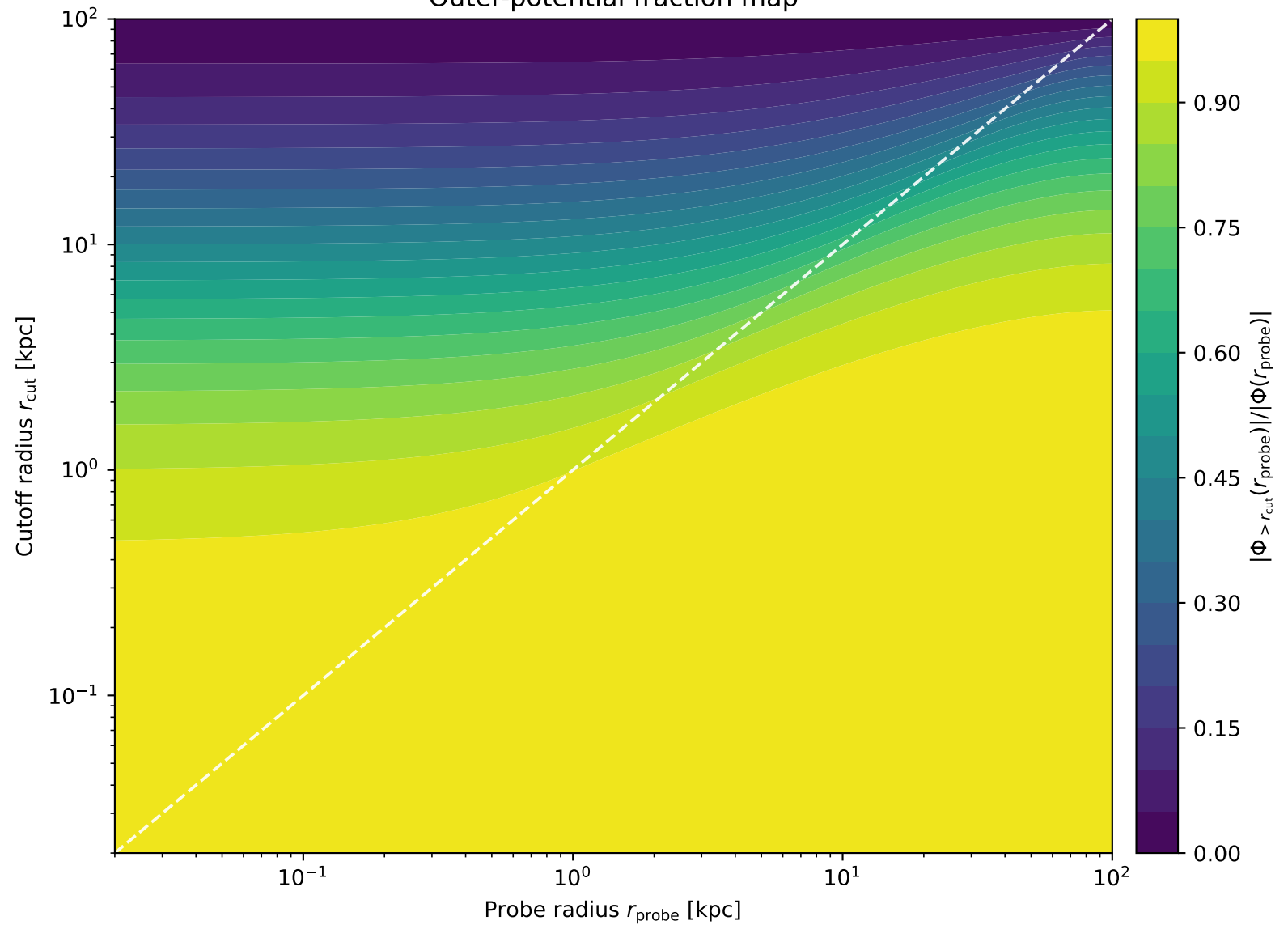
Outer-potential fraction map
