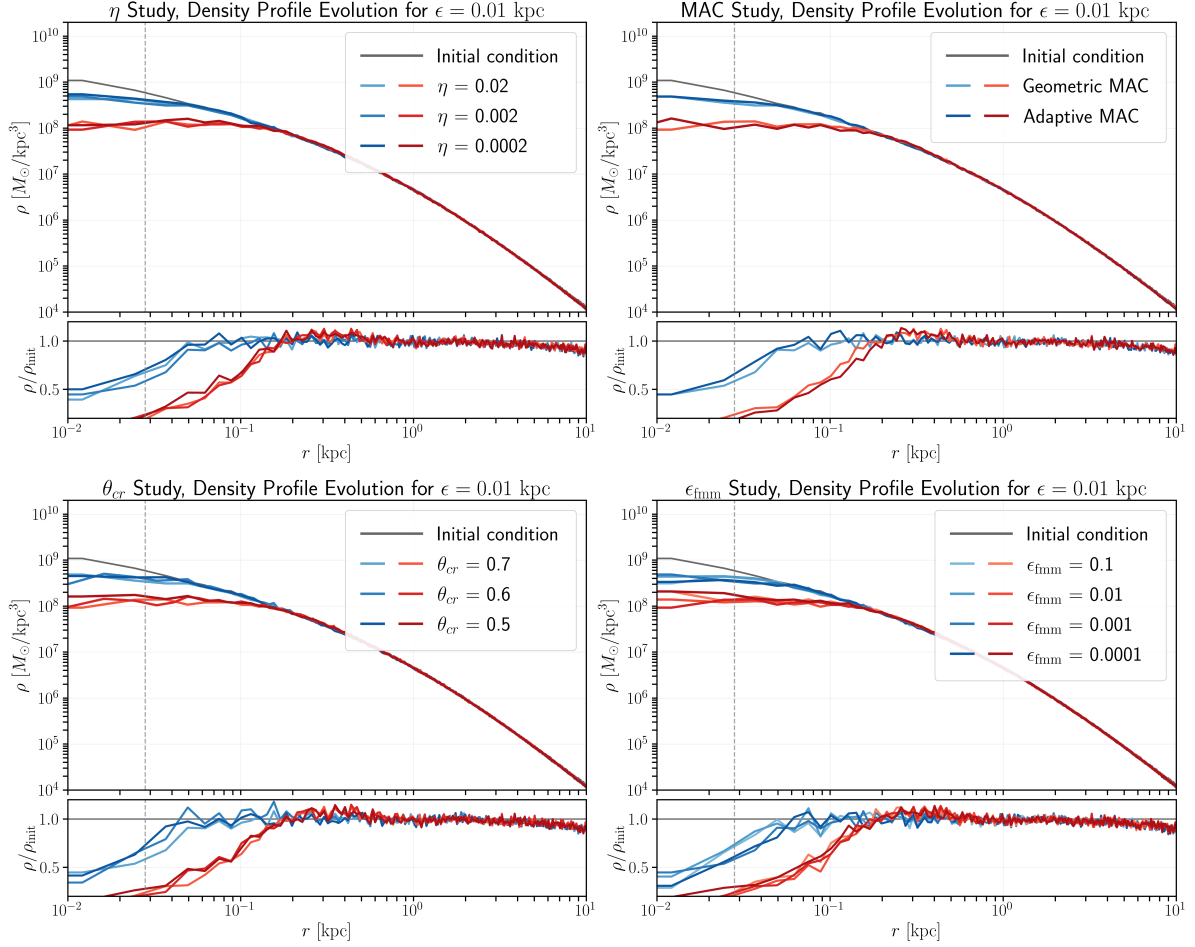
Figure 4.7: Self-gravity parameter study. Panels show the central-density evolution for the tested solver settings: top-left – timestep factor \eta ; top-right – MAC choice; bottom-left – geometric opening angle \theta_{\text{cr}} ; bottom-right – FMM tolerance \epsilon_{\text{fmm}} . In each panel blue curves correspond to 10 Gyr and red curves to 100 Gyr.
