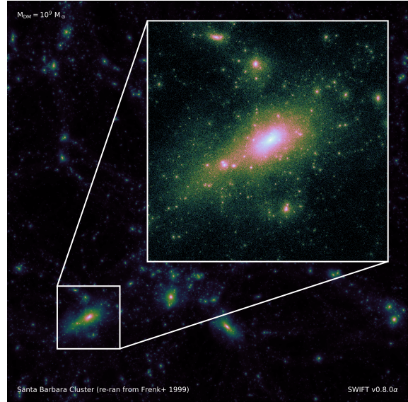
Santa-Barbara Cluster. A large-scale cluster formation snapshot from the Santa Barbara comparison suite. Image: Josh Borrow, SWIFT gallery.
