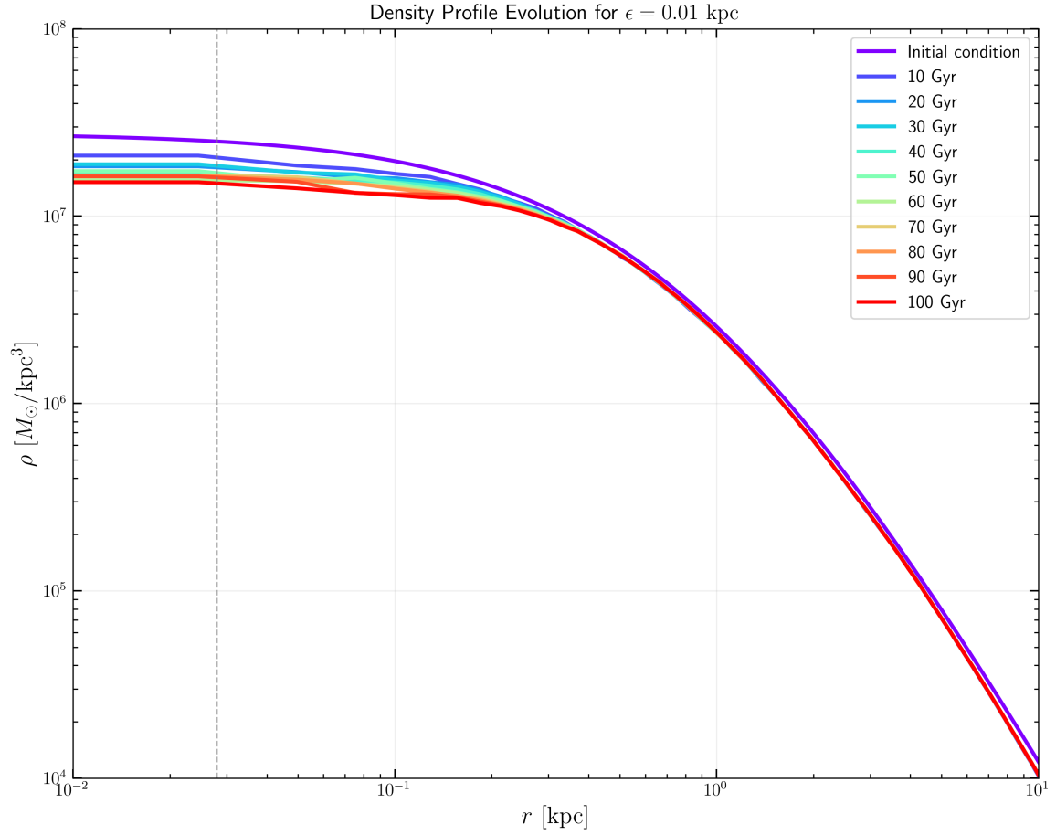
Figure 4.4: Core initial condition density-profile evolution. The cored halo also shows a decline in central density, although with a smaller amplitude than the cuspy case. This directly contradicts a simple expectation of core formation followed by stabilization.
