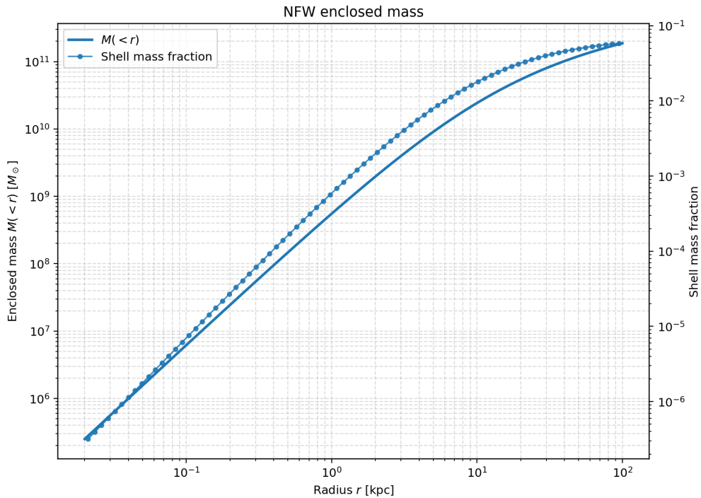
Figure 4.8: NFW enclosed mass and shell mass fraction. Left axis: monotonically increasing enclosed mass M(< r) with radius. Right axis: shell mass fraction per logarithmic shell.
