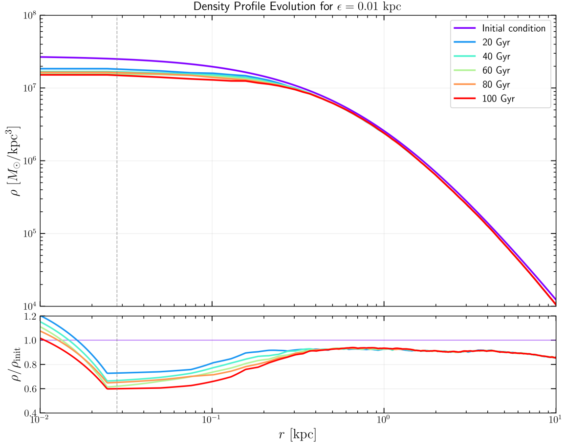
Figure 4.5: Core initial condition evolution with ratio to the initial state. The upper panel shows the density evolution over time. The lower panel shows the density ratio relative to the initial conditions.
