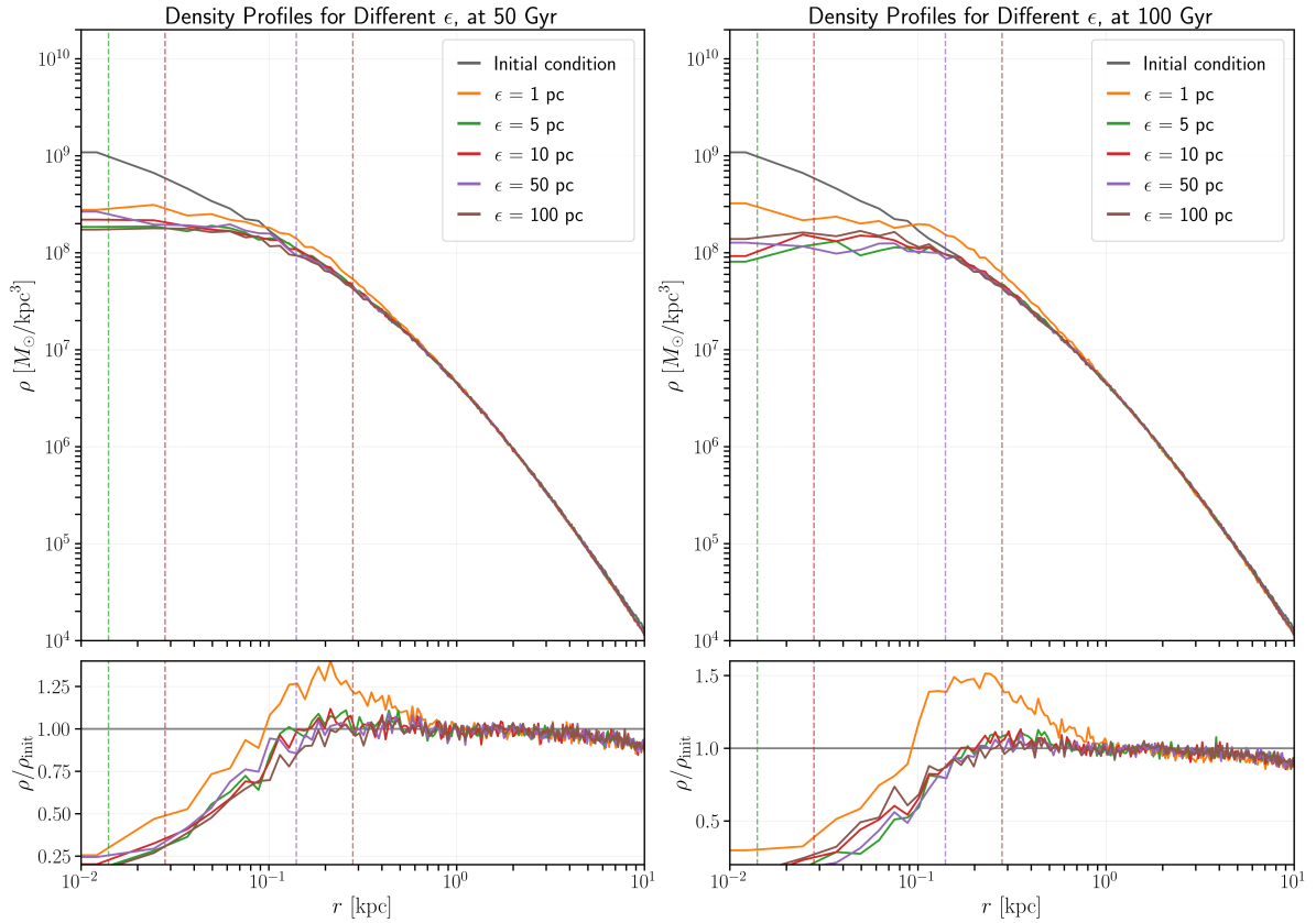
Figure 4.6: Softening study. Comparison of the same set of tested softening lengths at 50 Gyr (left) and 100 Gyr (right). The shorter-time view highlights the earlier evolution, while the longer-time view shows that the same hierarchy of softening runs follows the same qualitative trend. The smallest softening still shows a slight central-density increase close to the center, which is better interpreted as numerical heating than as a real improvement of the physical problem.
