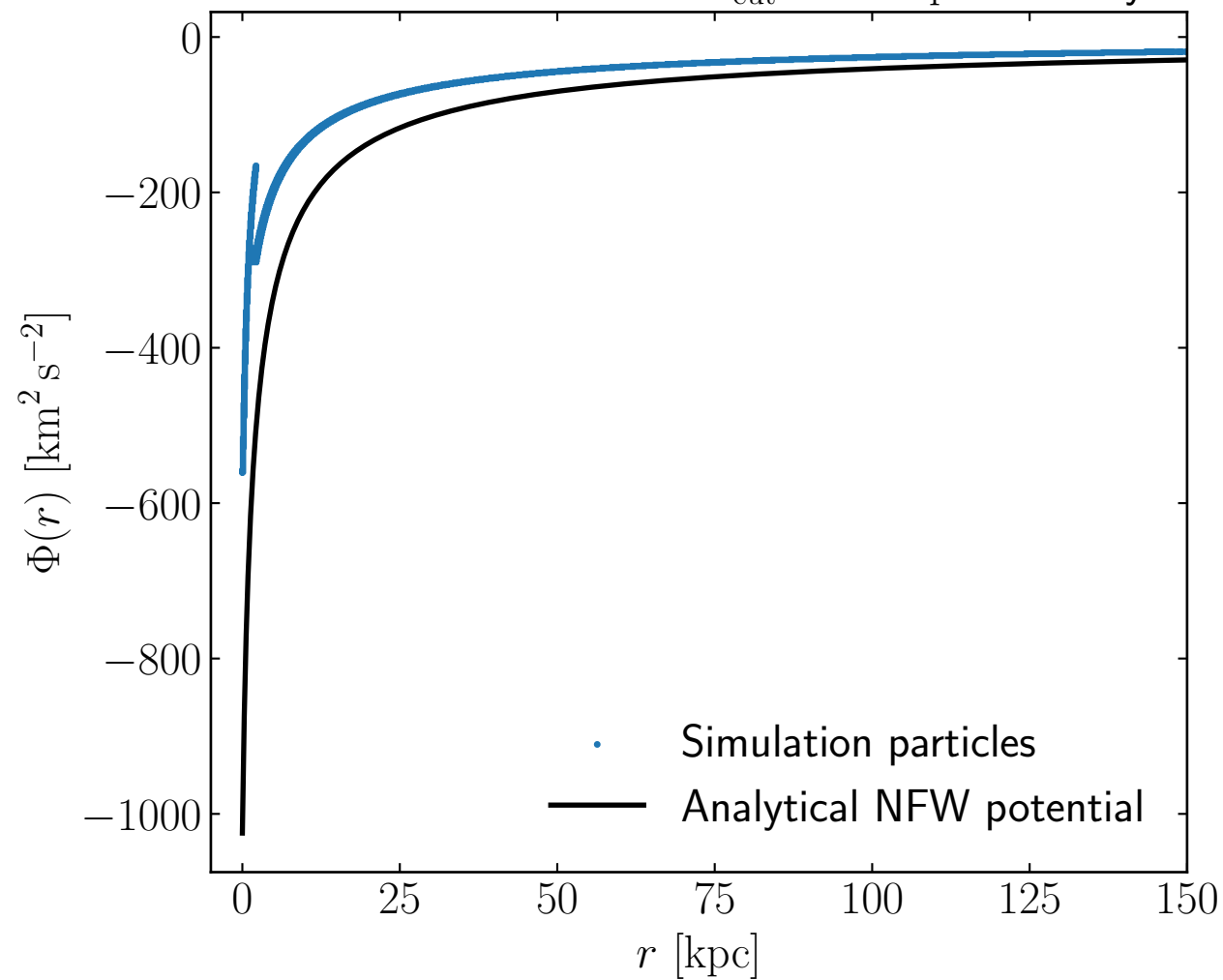
Potential distribution for R_{\text{cut}} = 2.0 kpc at 10 Gyr
