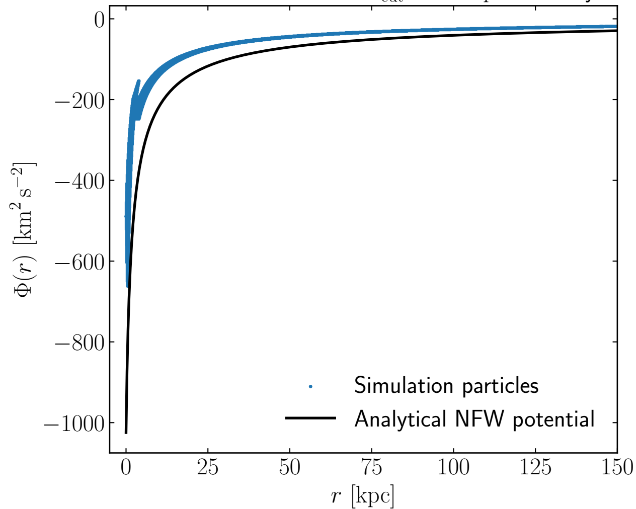
Potential distribution for R_{\text{cut}} = 3.0 kpc at 10 Gyr
