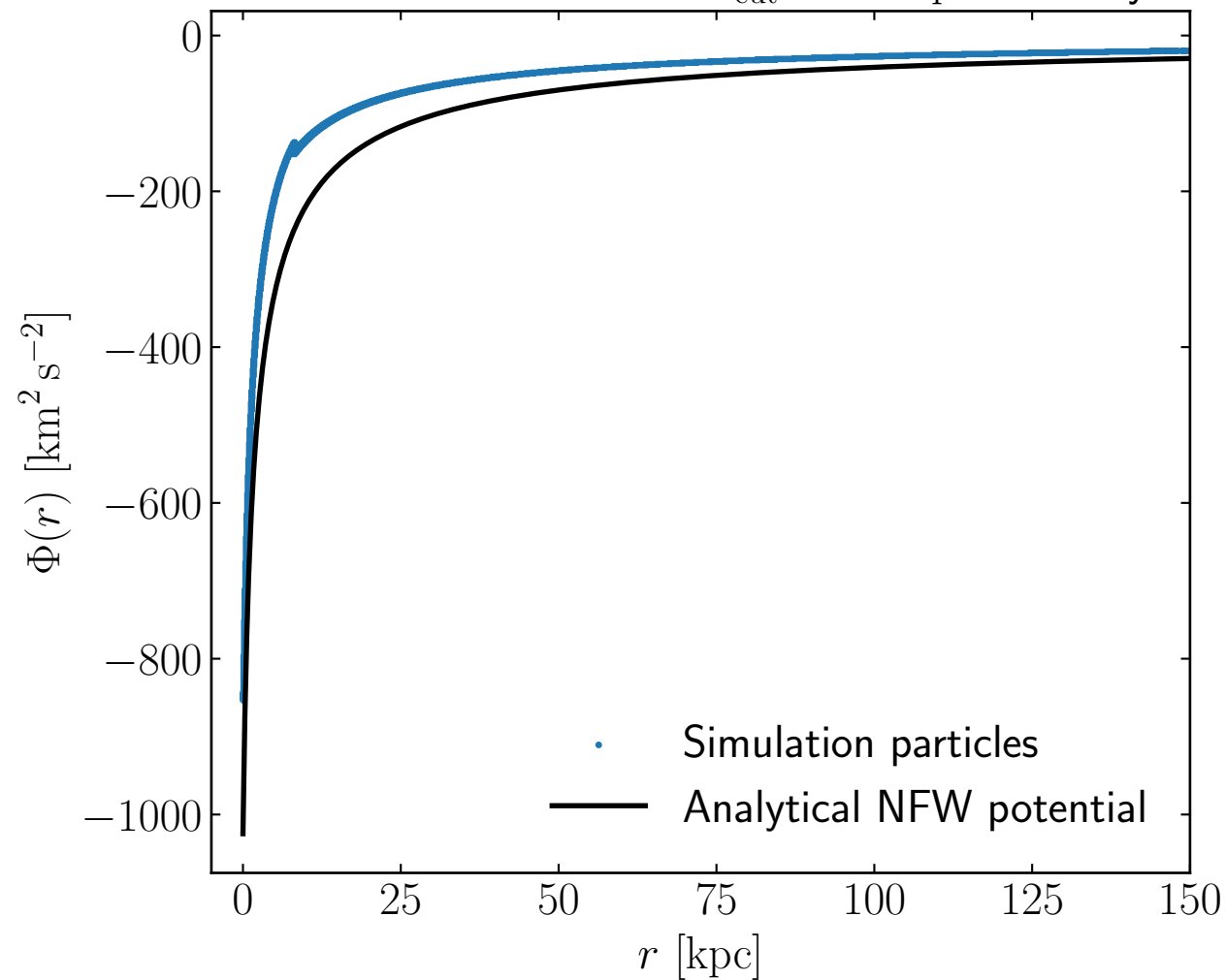
Potential distribution for R_{\text{cut}} = 8.0 kpc at 10 Gyr
