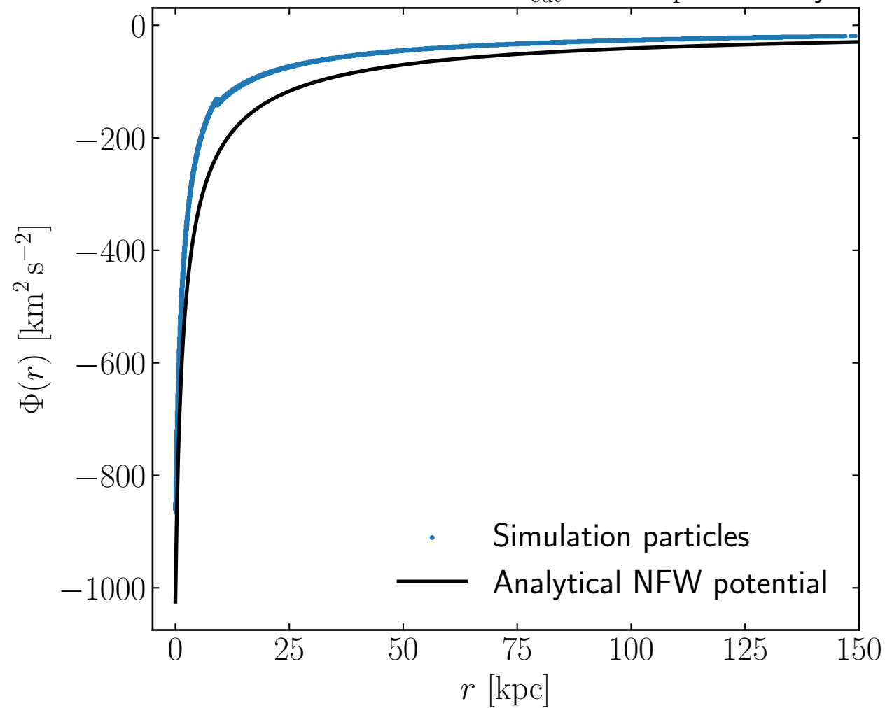
Potential distribution for R_{\text{cut}} = 9.0 kpc at 10 Gyr
