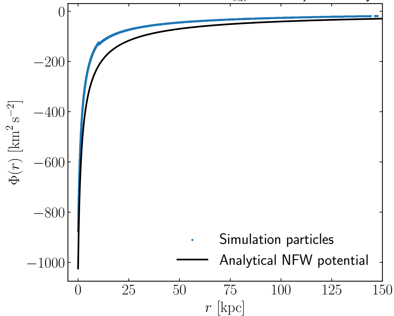
Potential distribution for R_{\text{cut}} = 10.0 kpc at 10 Gyr
