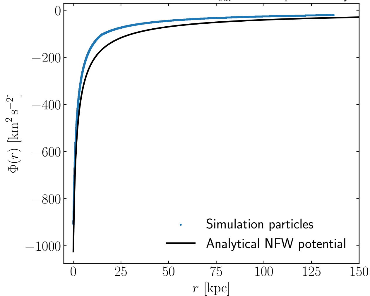
Potential distribution for R_{\text{cut}} = 15.0 kpc at 10 Gyr
