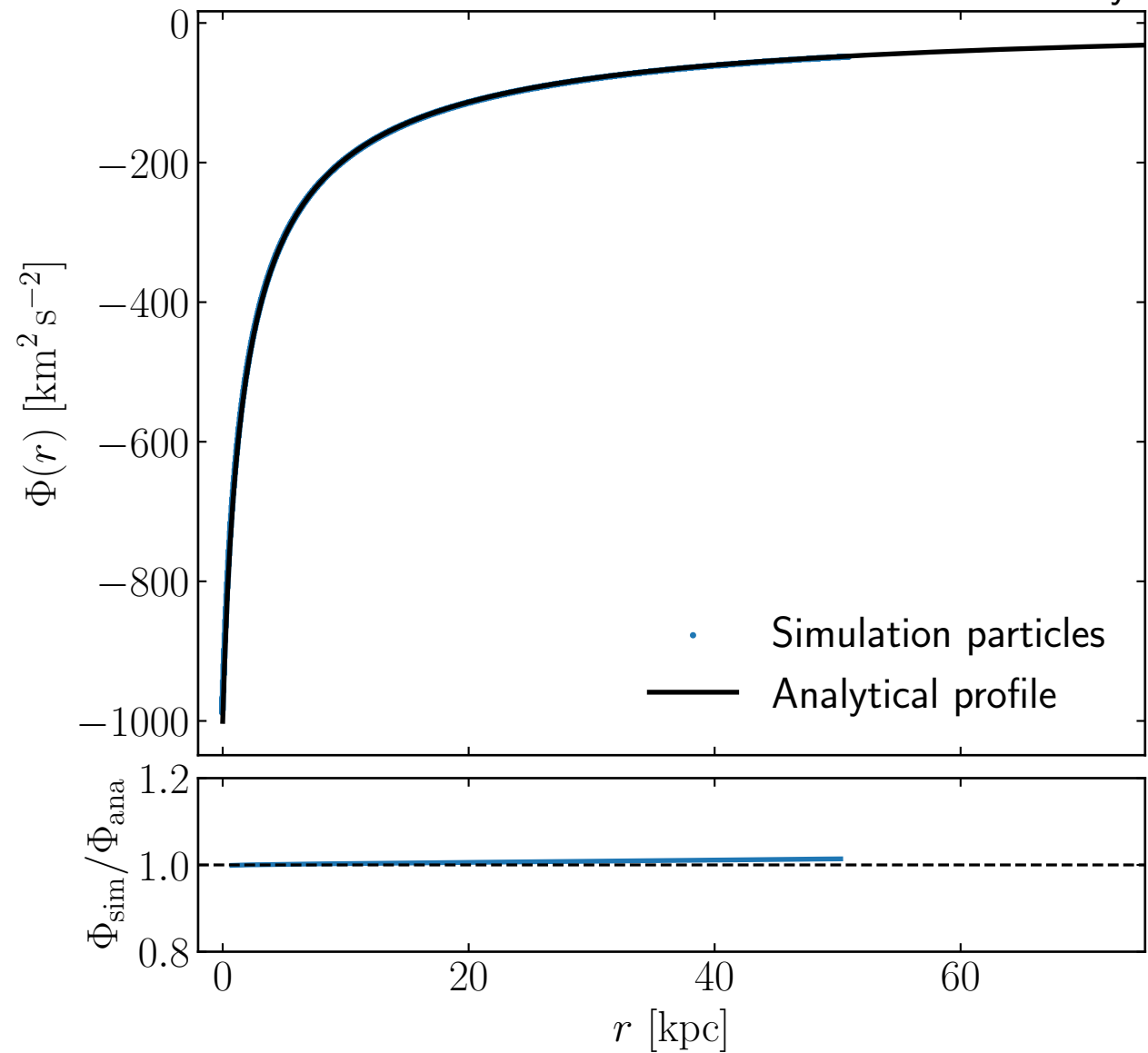
Potential distribution of baseline simulation at 100 Myr
