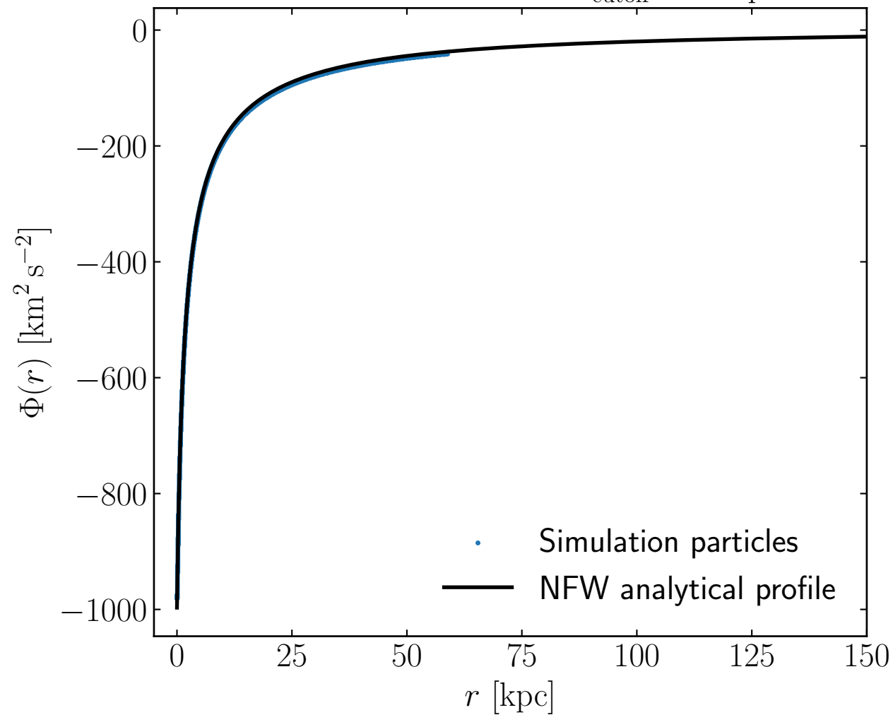
Potential distribution for r_{\text{cutoff}} = 50 \text{ kpc}
