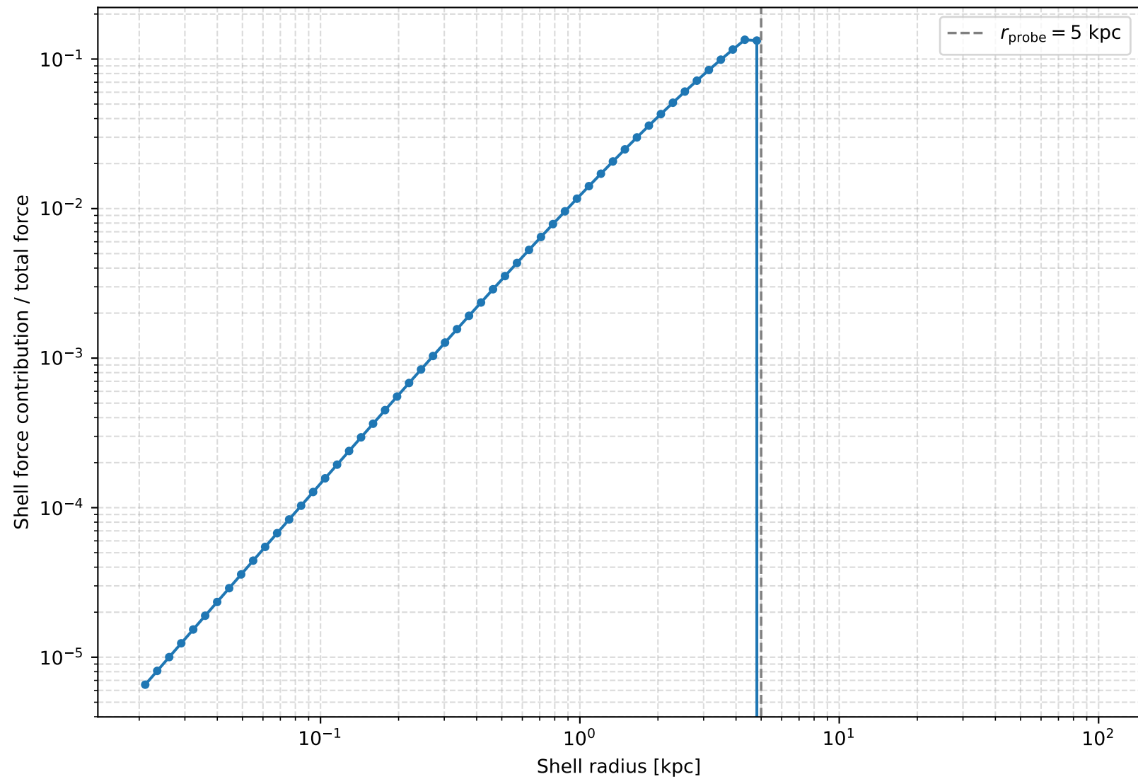
Force contribution at a finite inner radius
