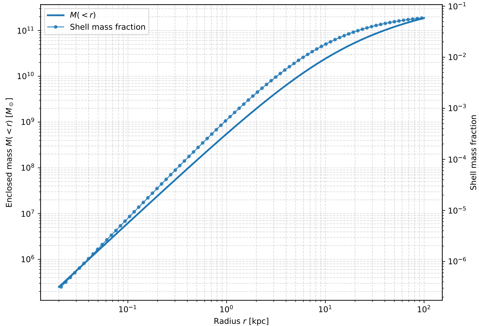
NFW enclosed mass
