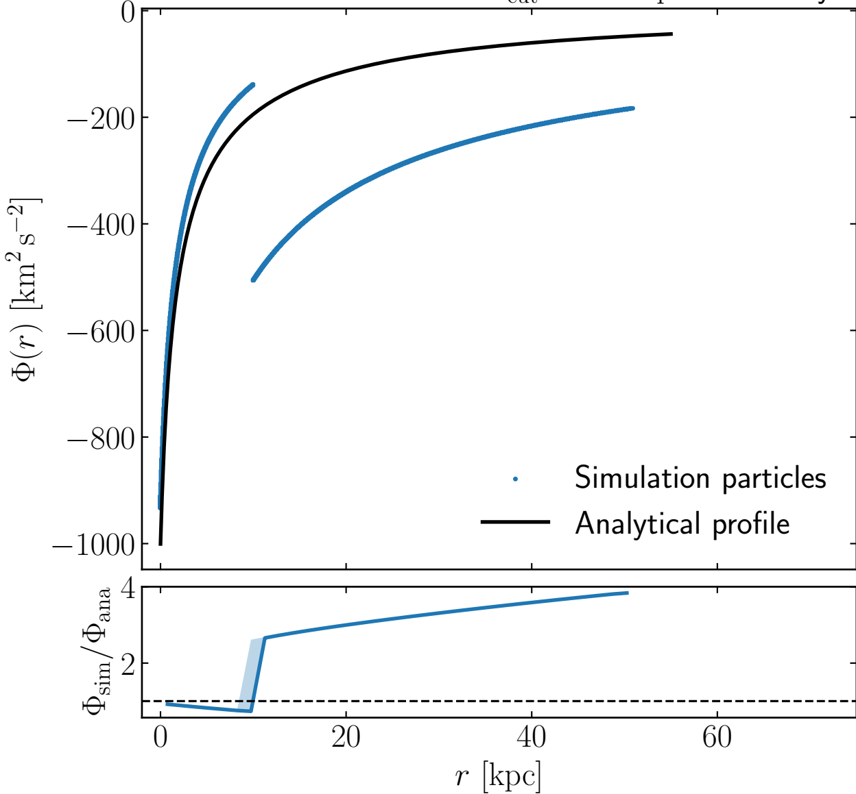
Potential distribution for R_{\text{cut}} = 10.0 \text{ kpc} at 100 Myr
