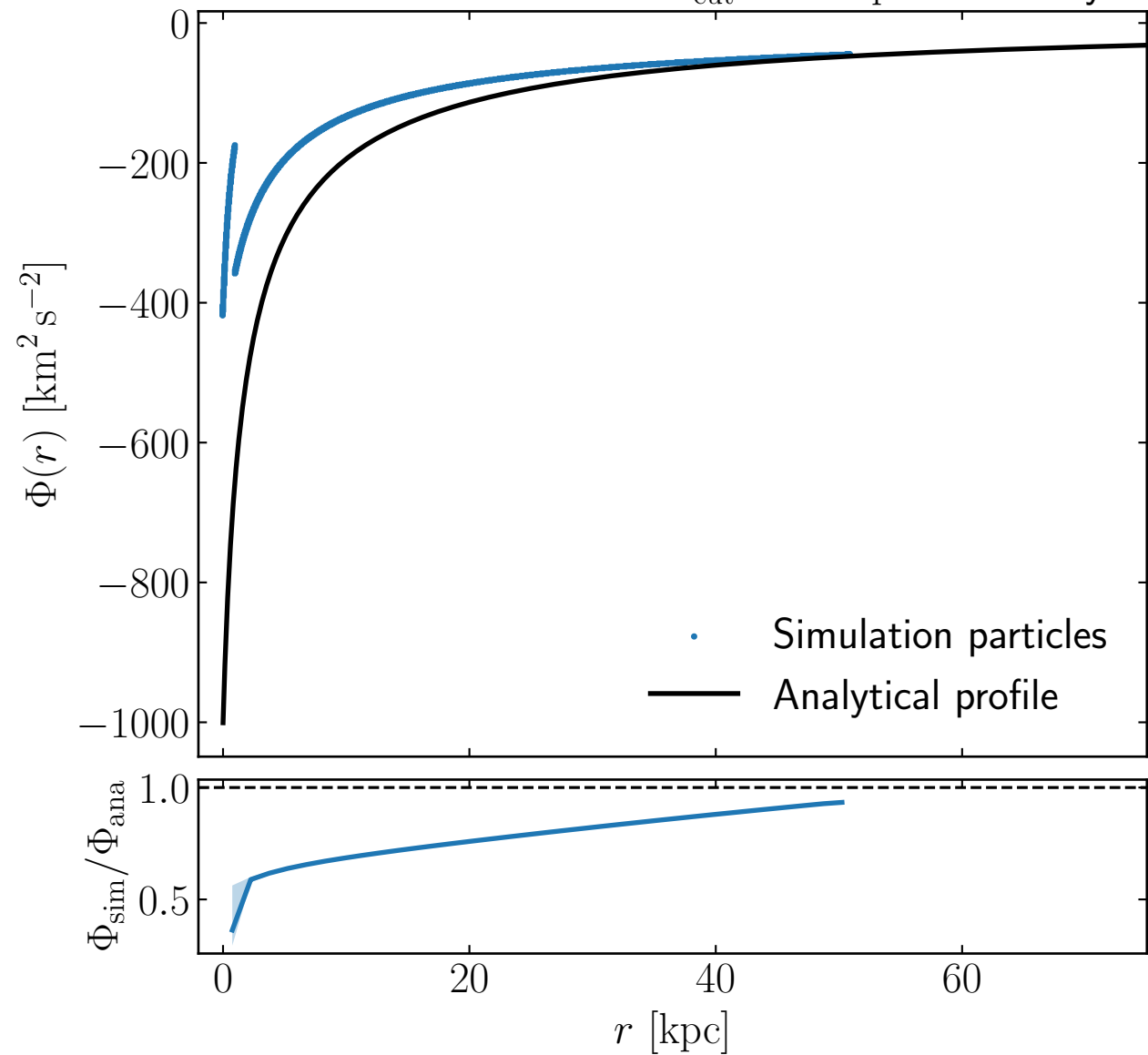
Potential distribution for R_{\text{cut}} = 1.0 \text{ kpc} at 100 Myr
