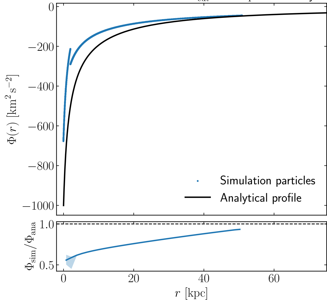
Potential distribution for R_{\text{cut}} = 2.0 \text{ kpc} at 100 Myr
