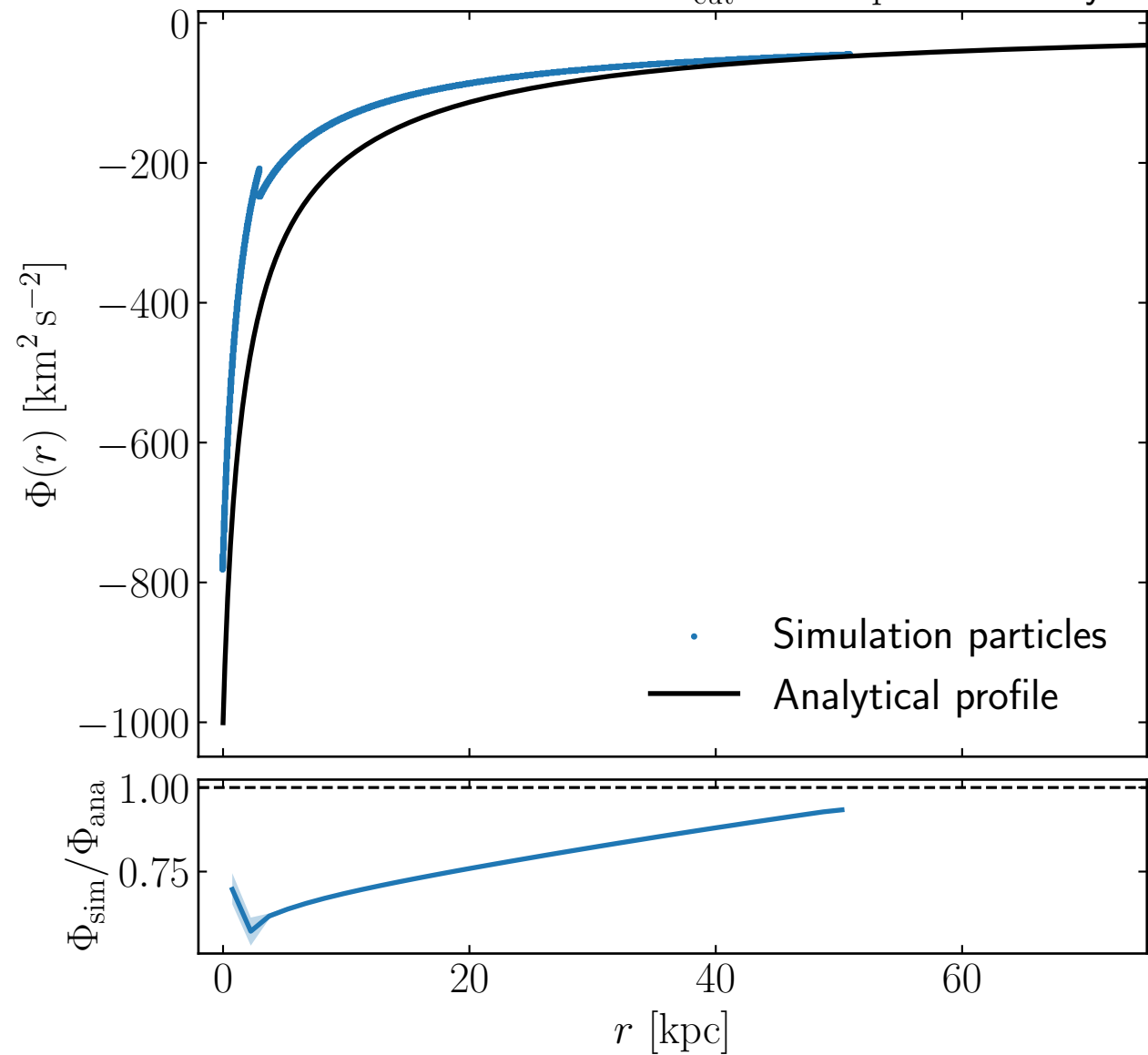
Potential distribution for R_{\text{cut}} = 3.0 \text{ kpc} at 100 Myr
