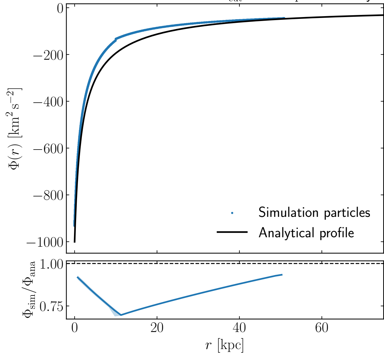
Potential distribution for R_{\text{cut}} = 10.0 \text{ kpc} at 100 Myr
