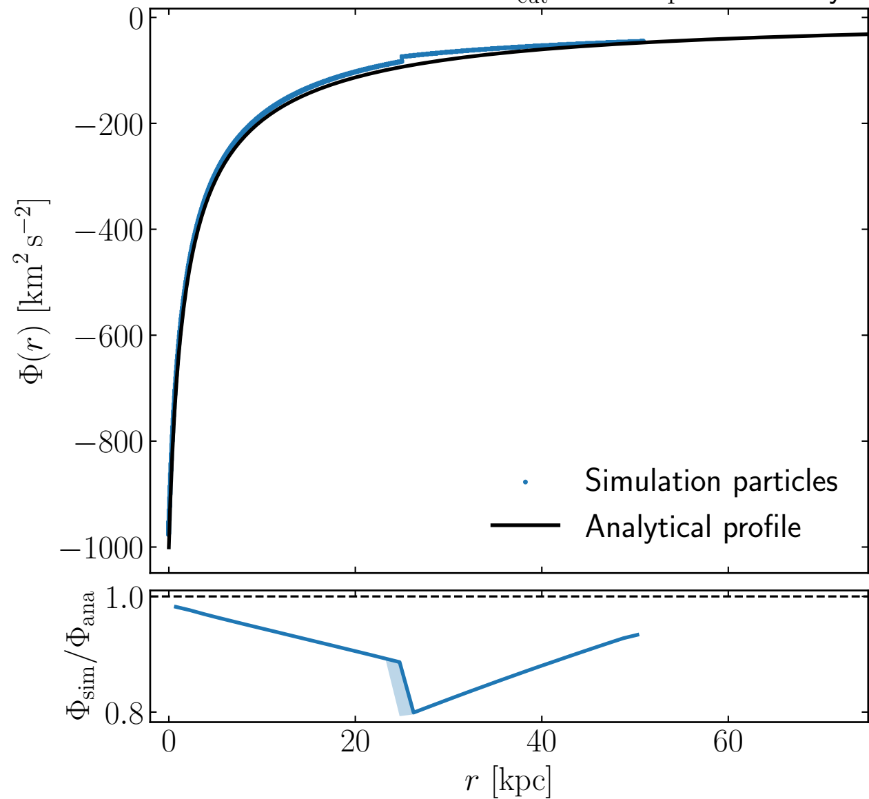
Potential distribution for R_{\text{cut}} = 25.0 \text{ kpc} at 100 Myr
