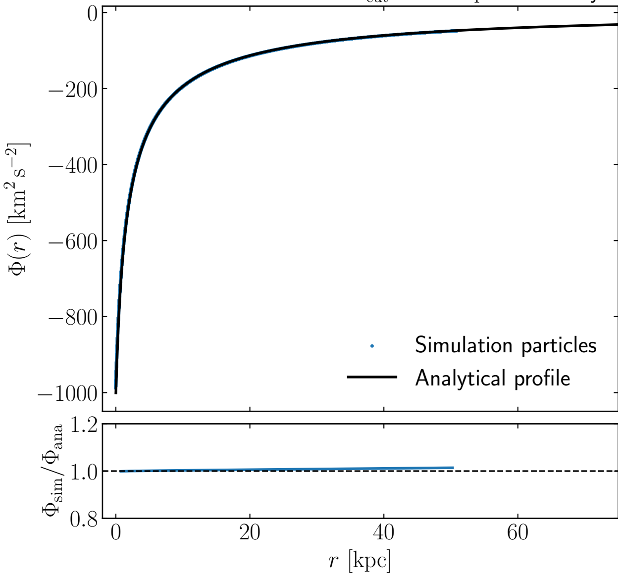
Potential distribution for R_{\text{cut}} = 50.0 \text{ kpc} at 100 Myr
