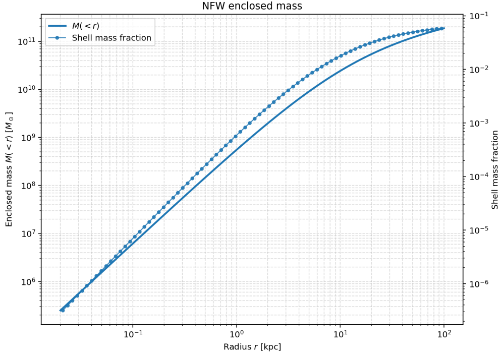
Figure 4.9: NFW enclosed mass and shell mass fraction. Left axis: monotonically increasing enclosed mass M(<r) with radius. Right axis: shell mass fraction per logarithmic shell.
