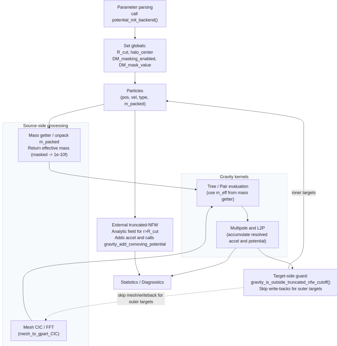
Figure 3.1: High-level control-flow schematic of the truncated-NFW implementation. The figure highlights the split between parameter initialization, source-side masking, gravity-kernel evaluation, target-side write-back suppression, and the external analytic field used for outer particles.
