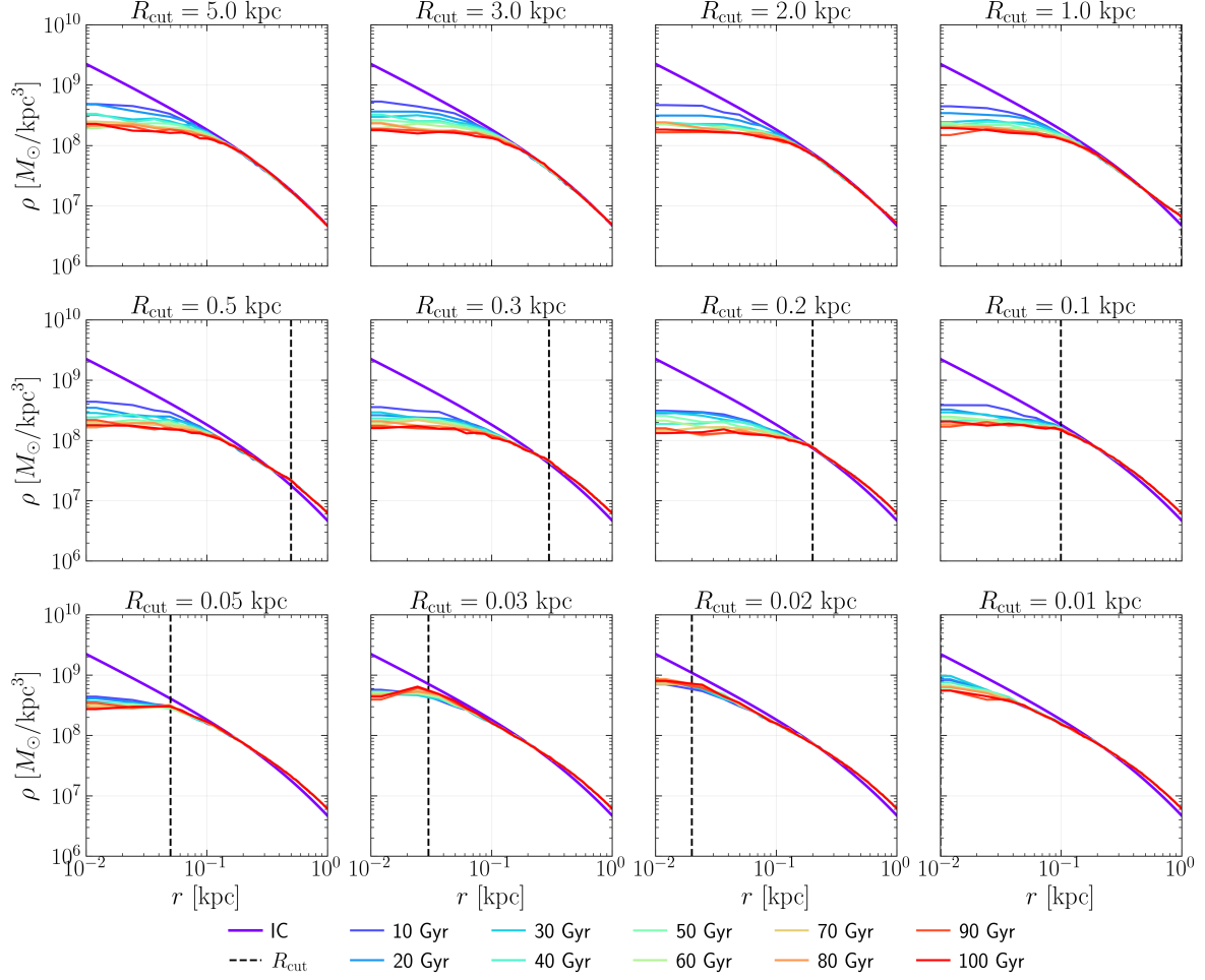
Figure 4.16: R_{\text{cut}} study large plot.
