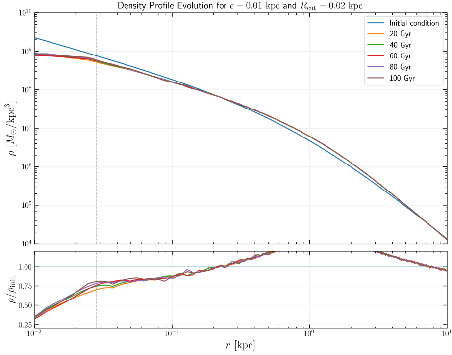
Figure C.5: Density profile evolution for the truncated-NFW test with cutoff at 0.02 kpc.
