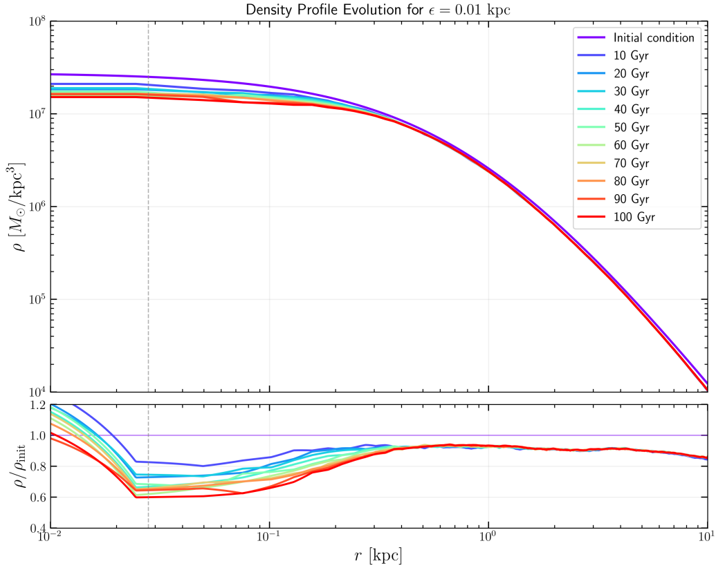
Figure 4.4: Core initial condition density-profile evolution with ratio to the initial state. The upper panel shows the density evolution over time. The lower panel shows the density ratio relative to the initial conditions.
