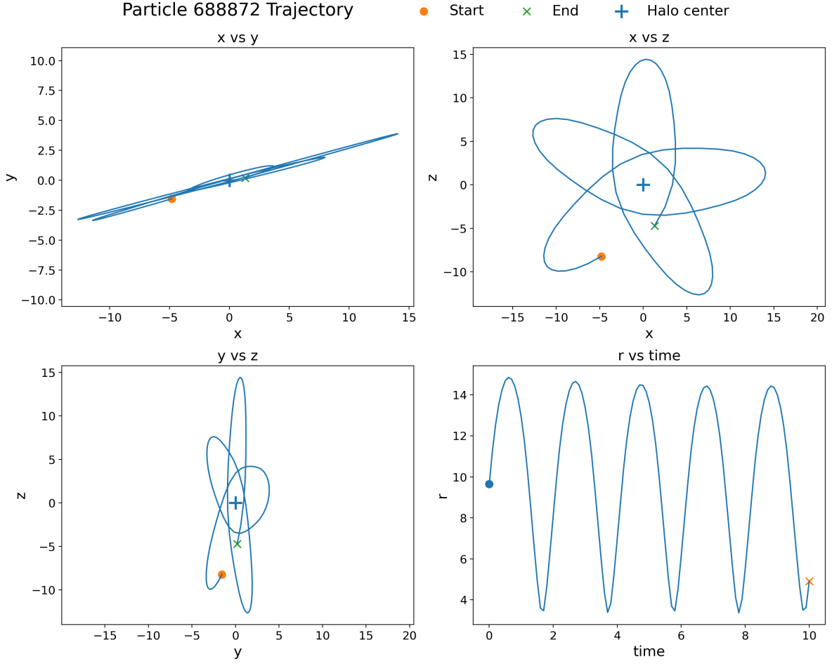
Figure 4.11: Orbit of example particle crossing the truncation boundary of R_{\text{cut}} = 10 kpc.
