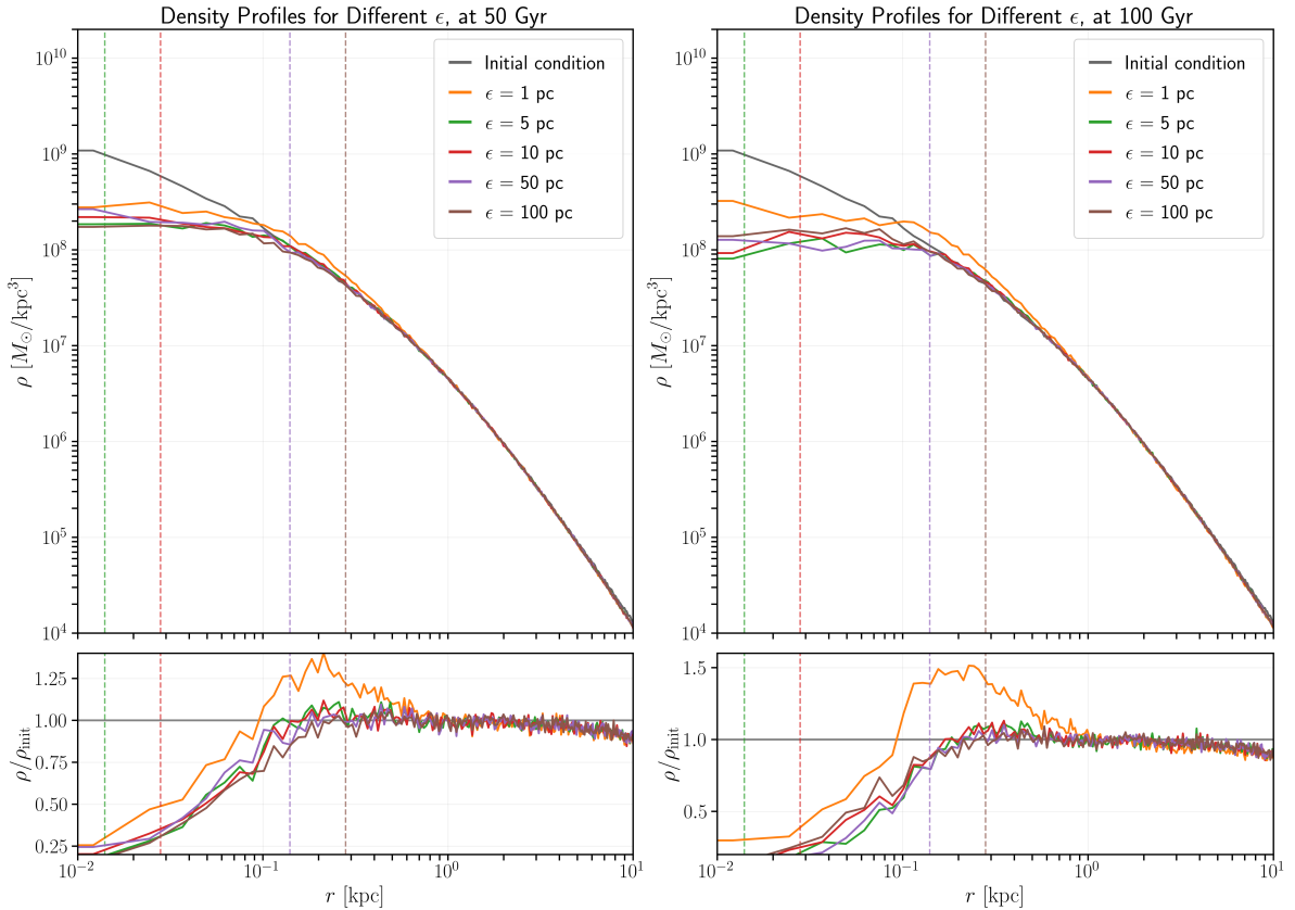
Figure 4.5: Softening study. Comparison of the same set of tested softening lengths ( \epsilon = 1, 5, 10, 50 , and 100 pc) at 50 Gyr (left) and 100 Gyr (right).
