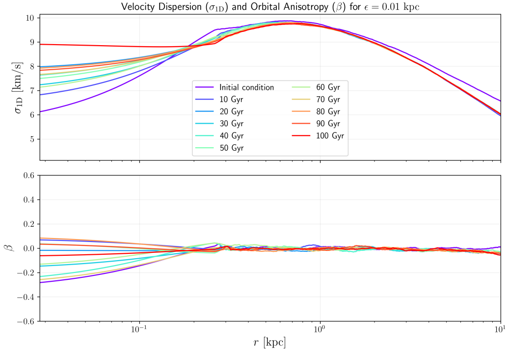
Figure 4.2: Velocity dispersion and orbital anisotropy evolution up to 100 Gyr for a softening length value of \epsilon = 0.01 kpc.
