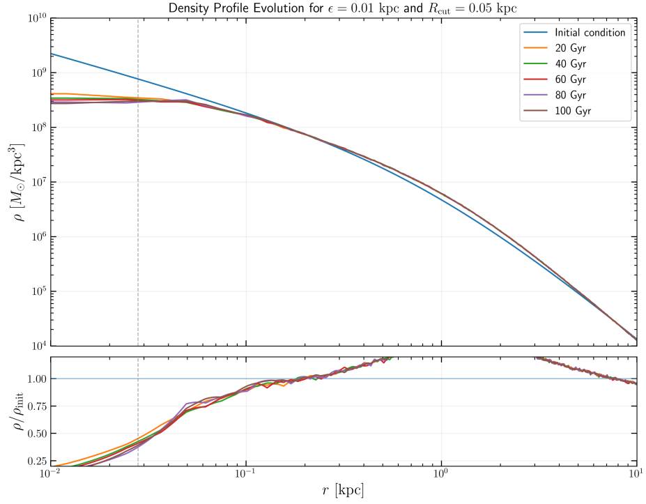
Figure C.3: Density profile evolution for the truncated-NFW test with cutoff at 0.05 kpc.
