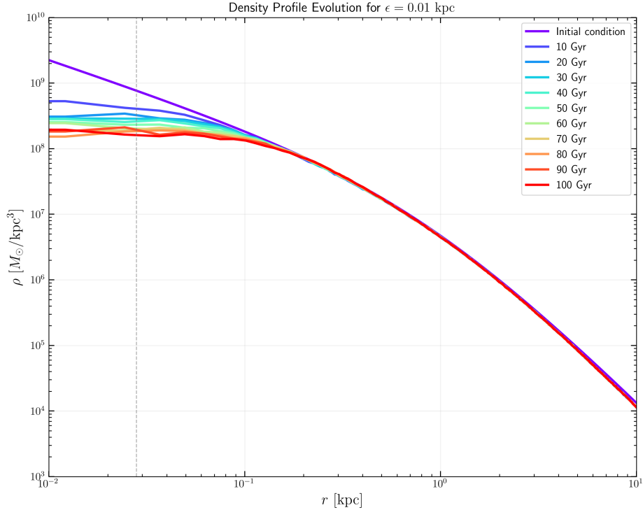
Figure 4.13: Density profile evolution of the hybrid model.
