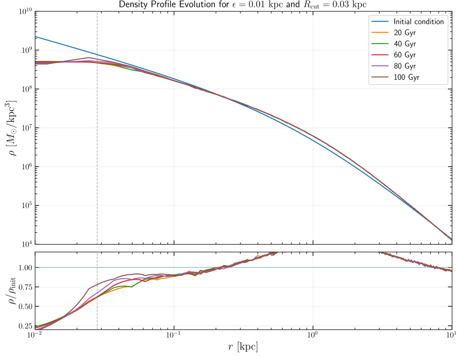
Figure C.4: Density profile evolution for the truncated-NFW test with cutoff at 0.03 kpc.
