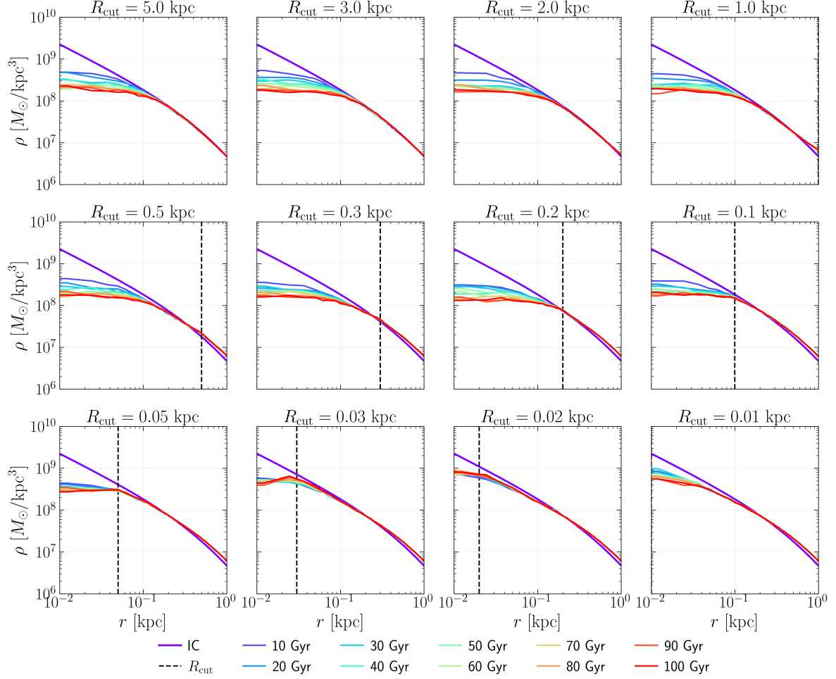
Figure 4.14: R_{\text{cut}} study large plot.
