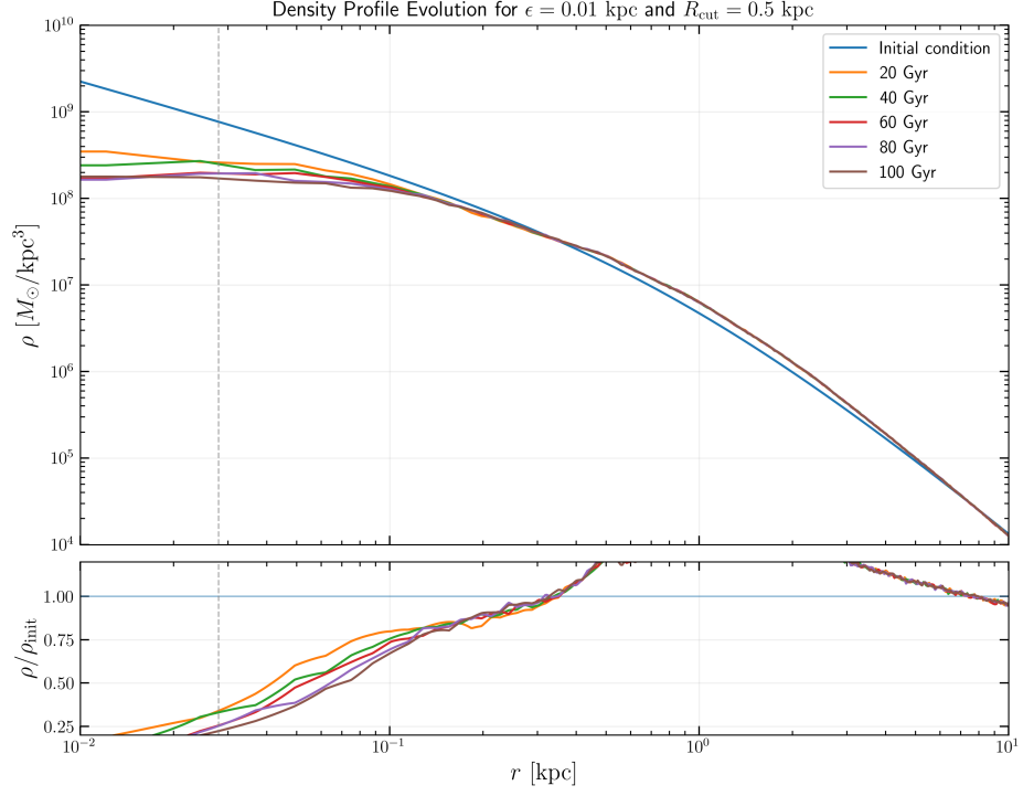
Figure C.2: Density profile evolution for the truncated-NFW test with cutoff at 0.5 kpc.
