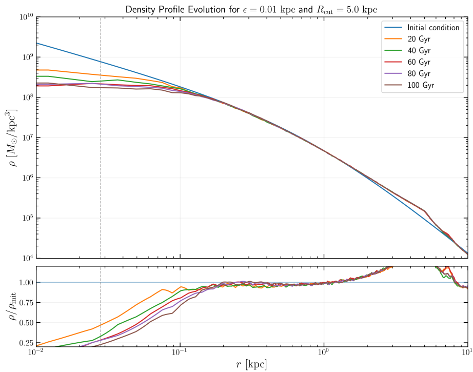
Figure C.1: Density profile evolution for the truncated-NFW test with cutoff at 5 kpc.
