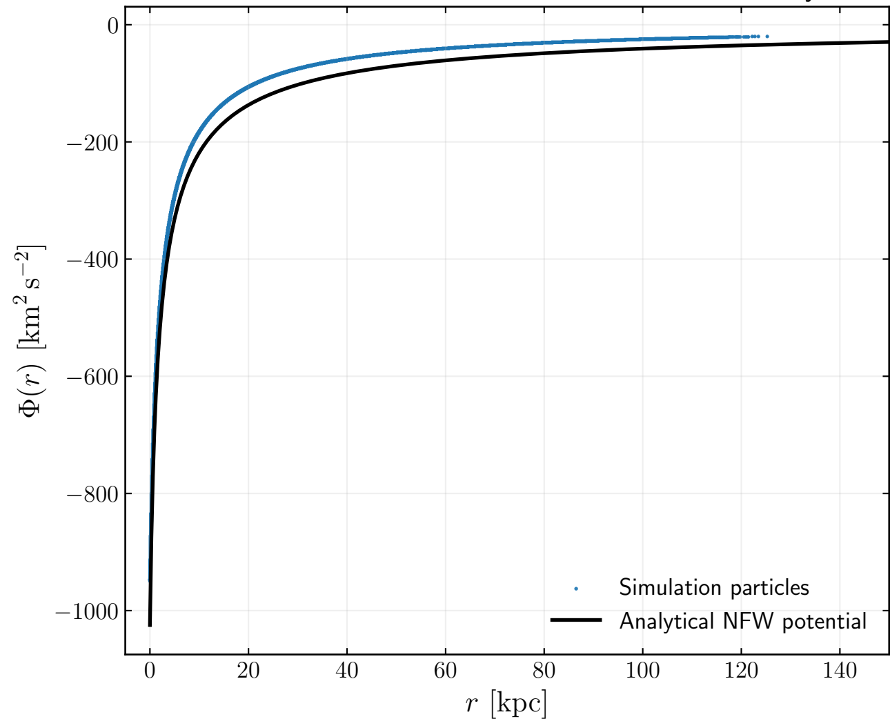
Potential distribution of baseline simulation at 10 Gyr
