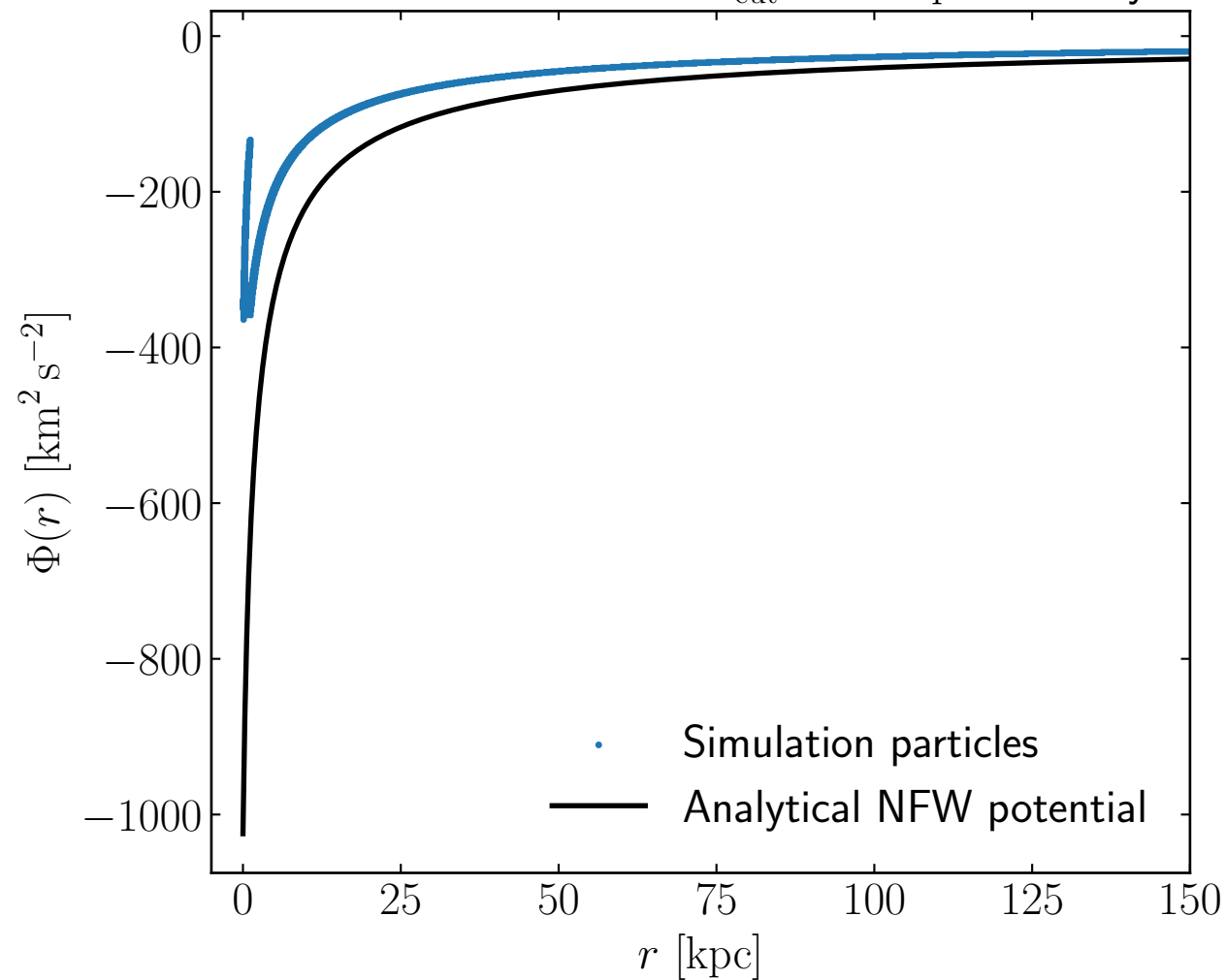
Potential distribution for R_{\text{cut}} = 1.0 kpc at 10 Gyr
