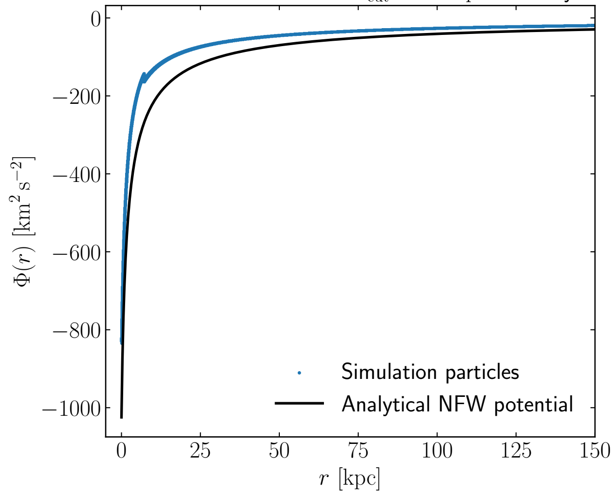
Potential distribution for R_{\text{cut}} = 7.0 kpc at 10 Gyr
