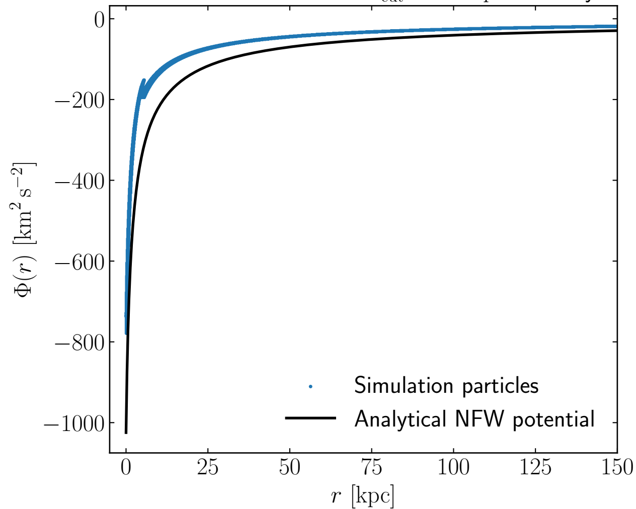
Potential distribution for R_{\text{cut}} = 5.0 kpc at 10 Gyr
