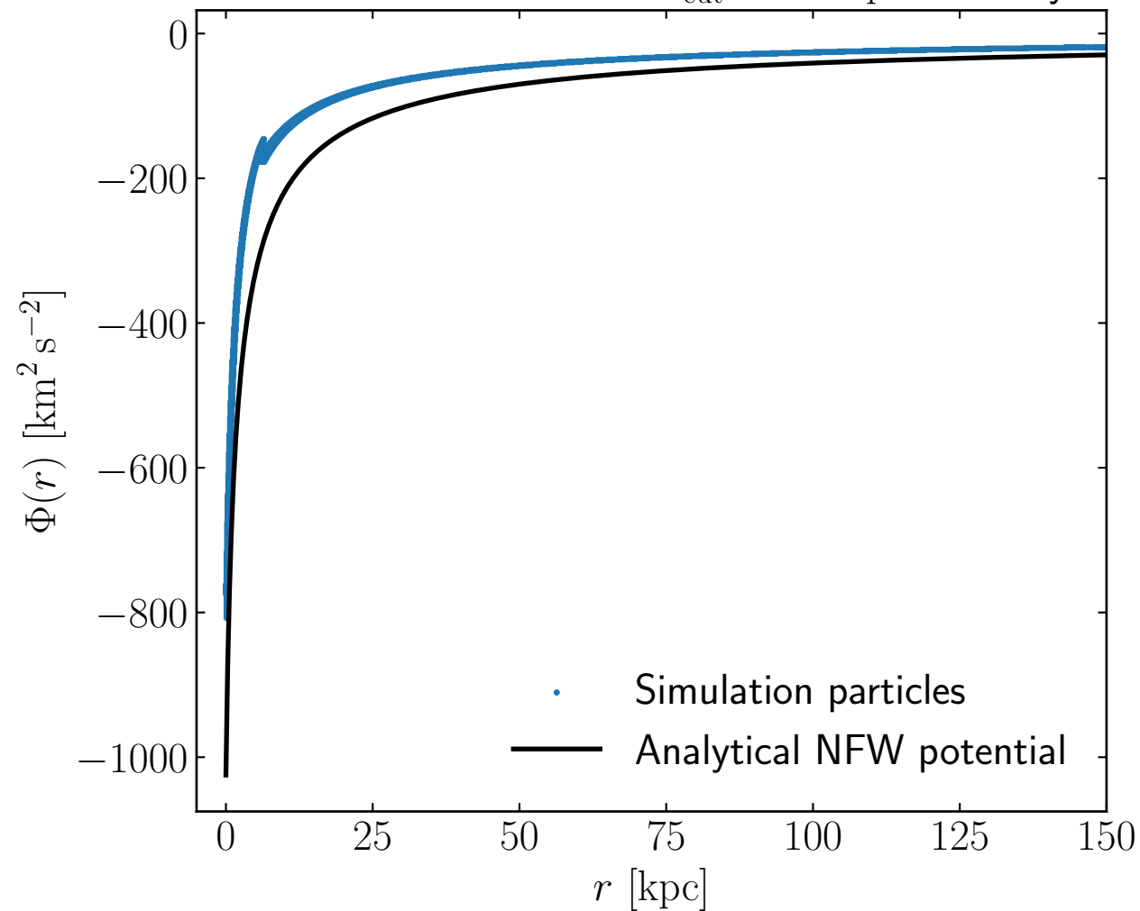
Potential distribution for R_{\text{cut}} = 6.0 kpc at 10 Gyr
