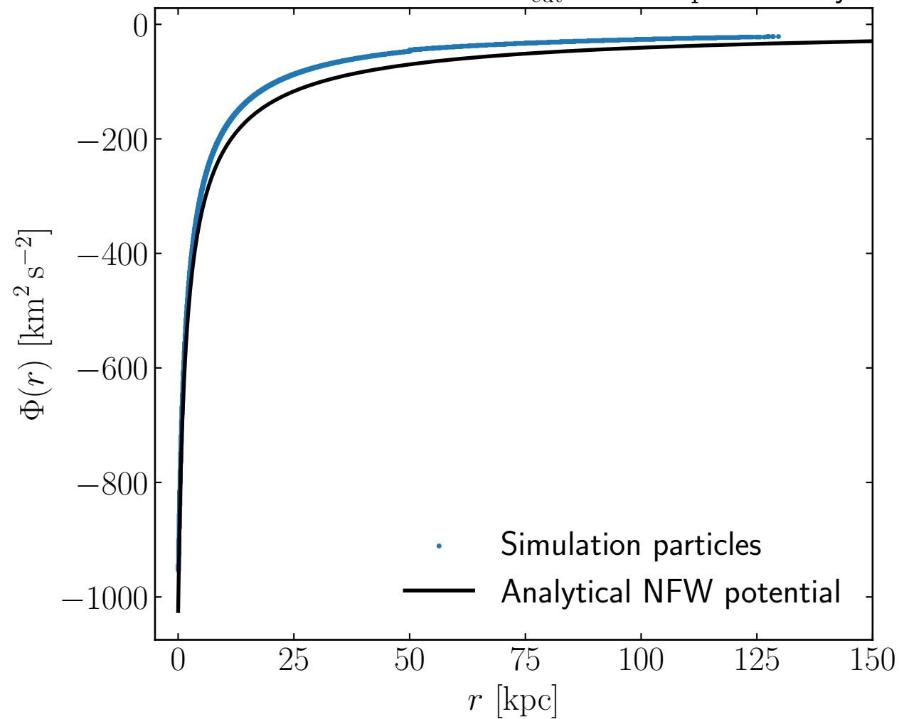
Potential distribution for R_{\text{cut}} = 50.0 kpc at 10 Gyr
