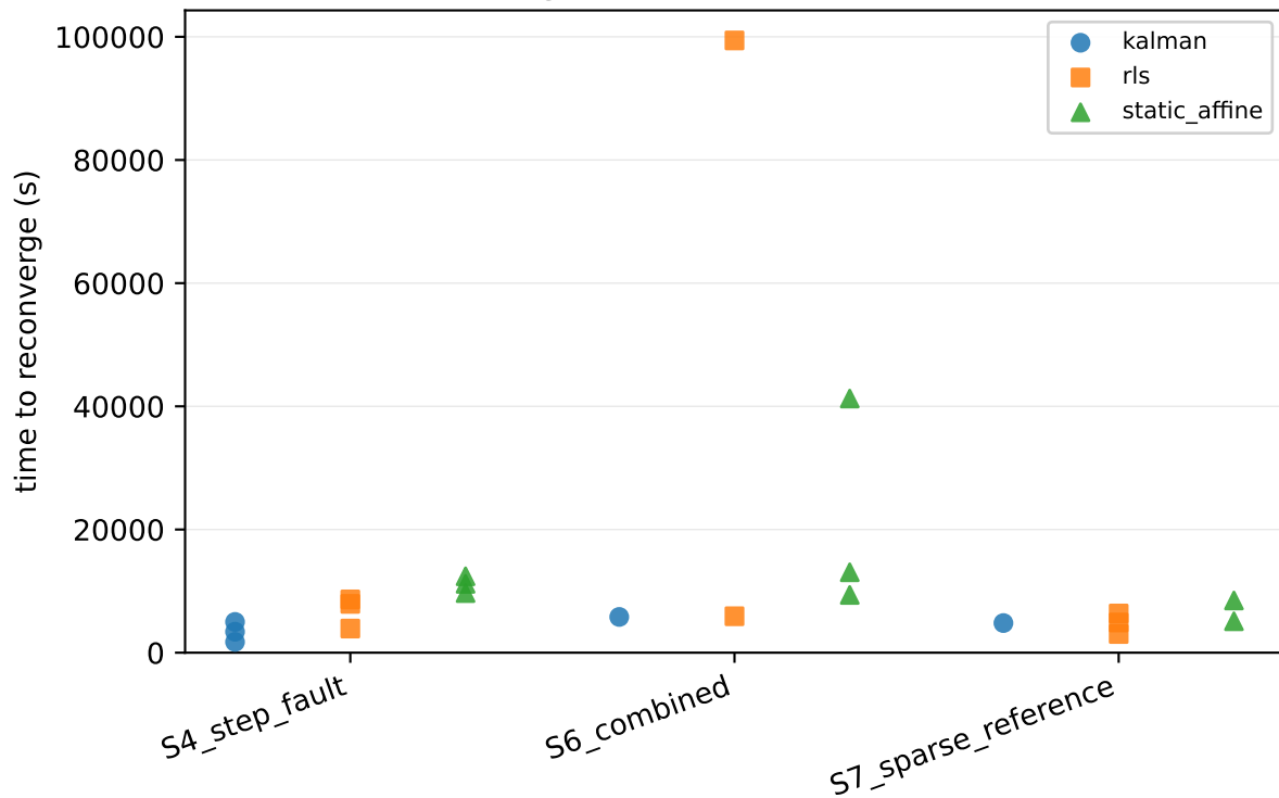
reconvergence [ladder -- 63 of 63 runs]
