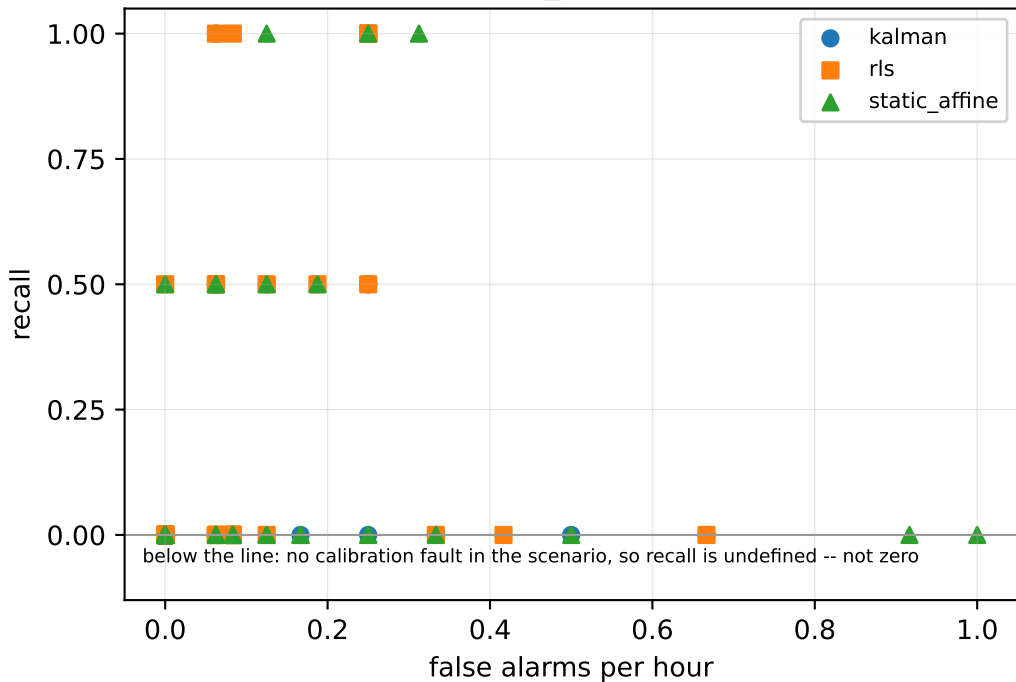
detectors [reference_rate -- 180 of 180 runs]
