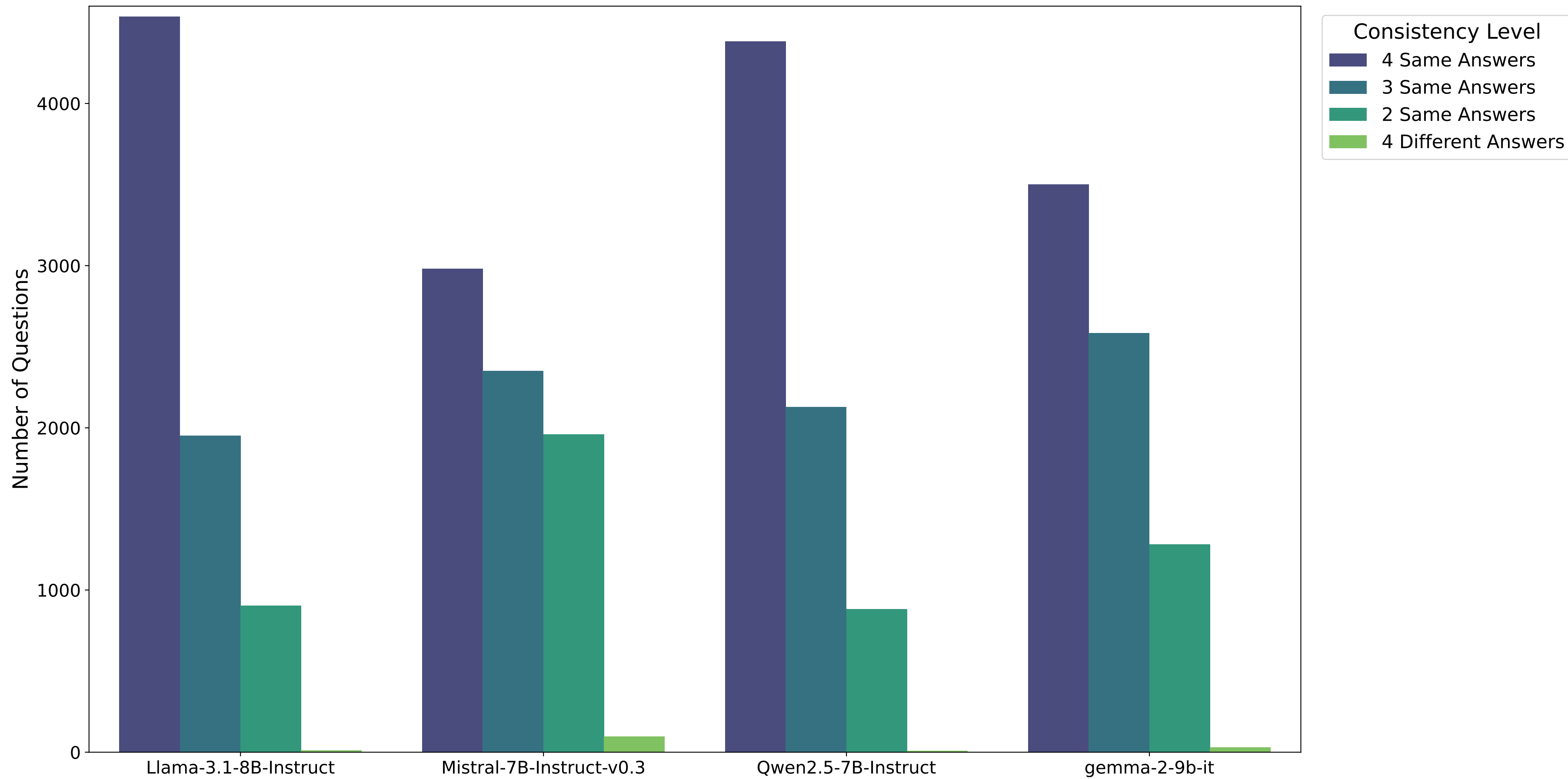
Consistency Across 4 Prompts: Shuffled Answer Options (Absolute Count) - Instruction-Tuned Models
