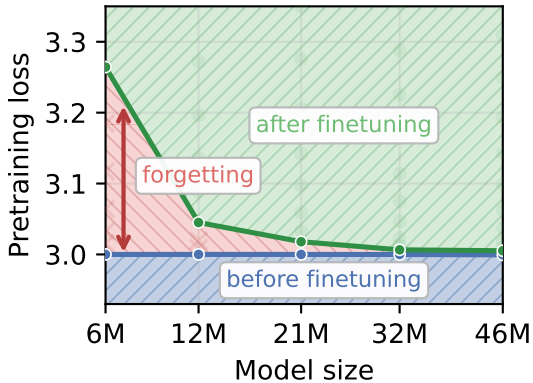
Larger models forget less
