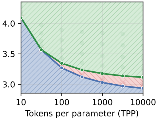
Longer pretraining increases forgetting
