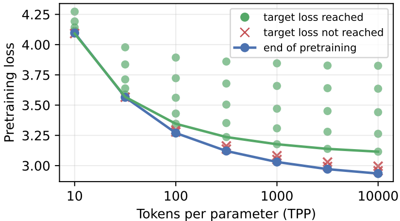
Longer pretraining increases forgetting
