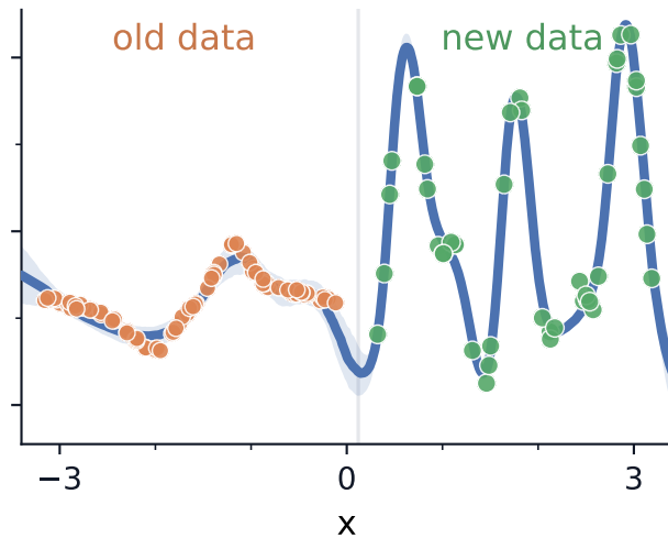
Finetuning w/ KL regularization
