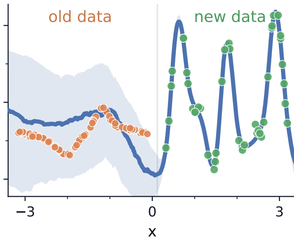
Finetuning on new data only
