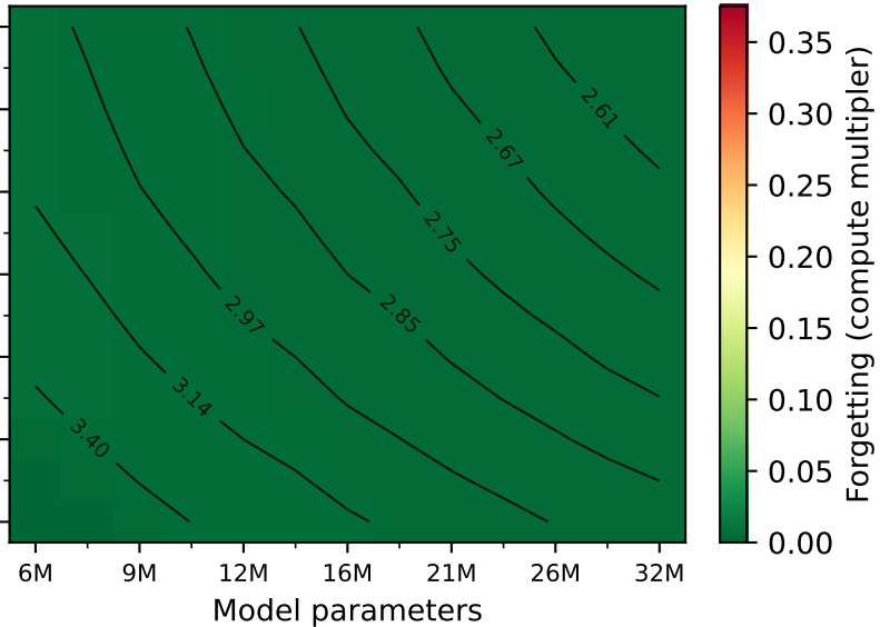
KL regularization
