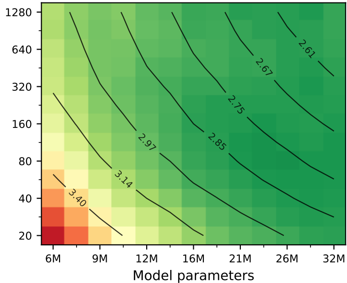
No regularization
