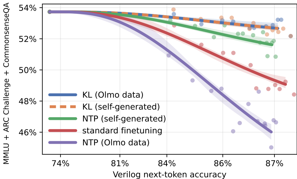
Avg. benchmark accuracy MMLU + ARC Challenge + CommonsenseQA
