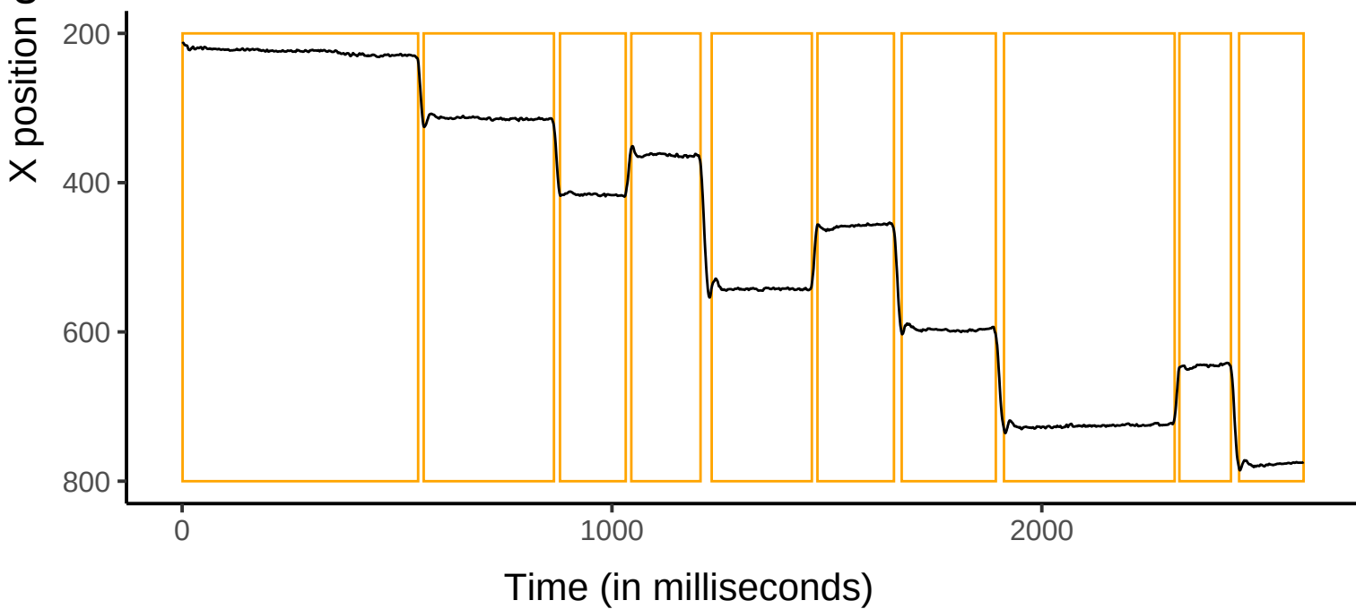
Engbert & Kliegl (2003) saccade detection algorithm ( \lambda = 12 )
