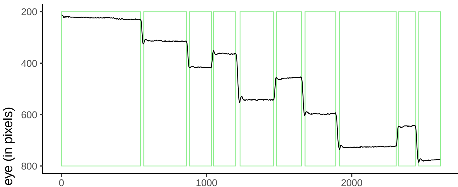
Engbert & Kliegl (2003) saccade detection algorithm ( \lambda = 12 )
