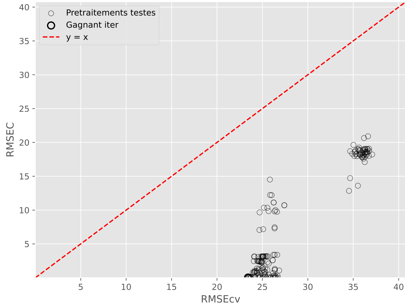
Overfitting pretraitements (Iter 5)
