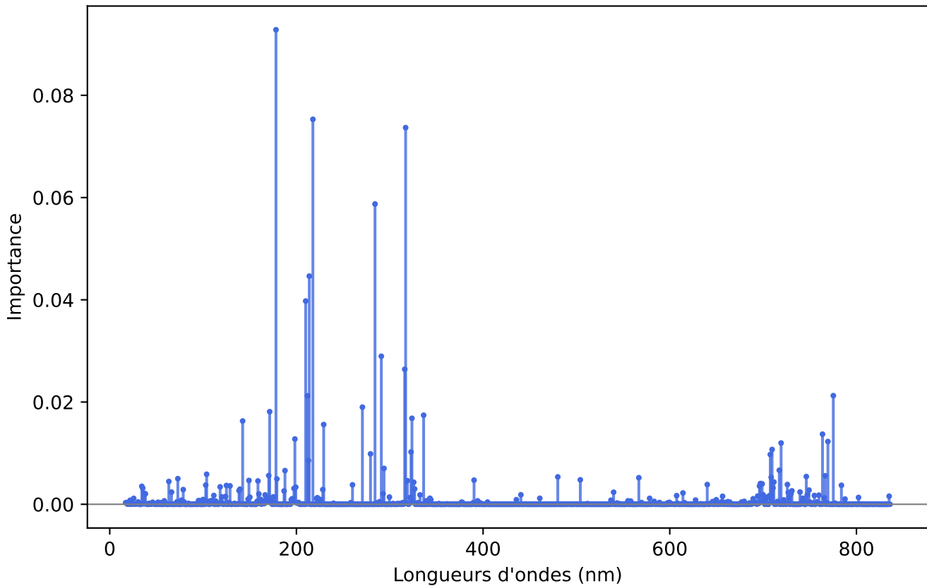
XGB Importance Variables (Iter 5)
