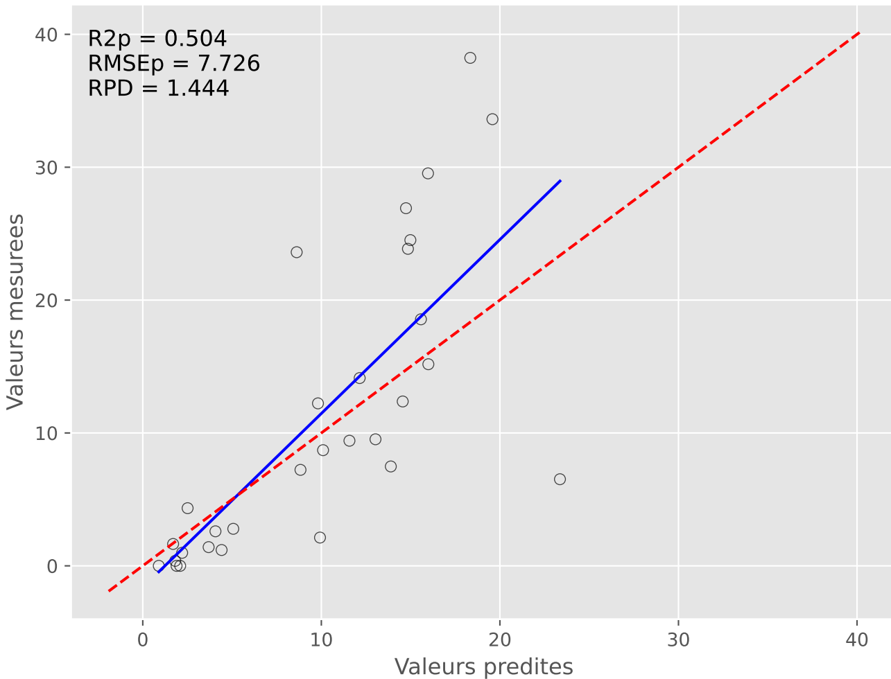
Predictions vs Mesures (Iter 7)
