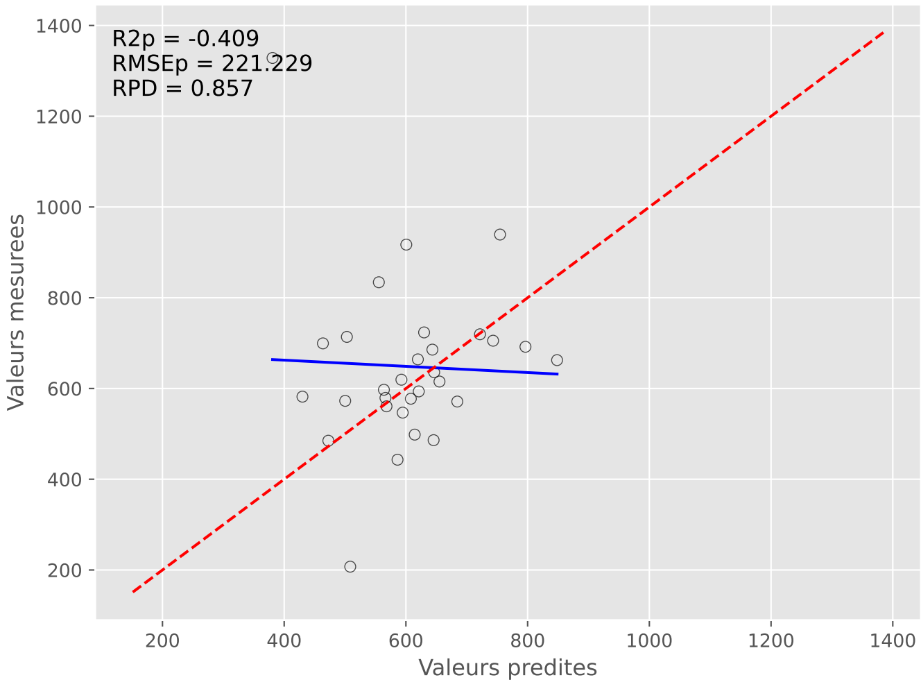
Predictions vs Mesures (Iter 3)
