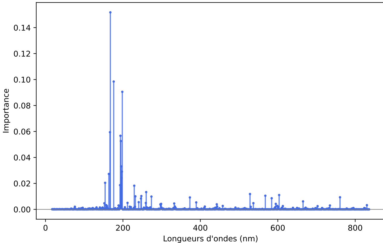
XGB Importance Variables (Iter 1)
