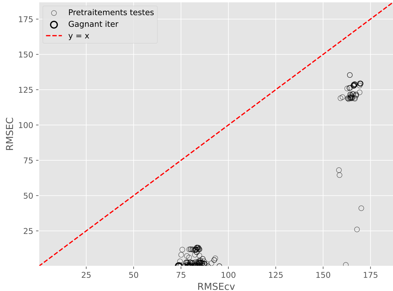
Overfitting pretraitements (Iter 1)
