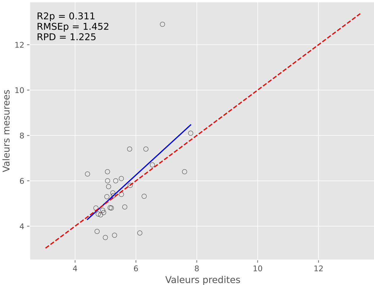
Predictions vs Mesures (Iter 7)
